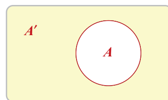
Complement
