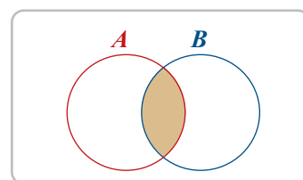
Intersection
