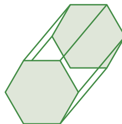
Hexagonal prism
