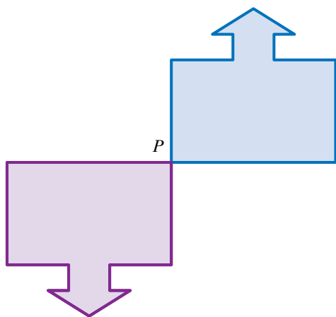
Rotation around P through 180^\circ in a clockwise direction
