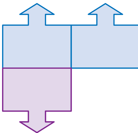
Reflection followed by translation or two reflections
