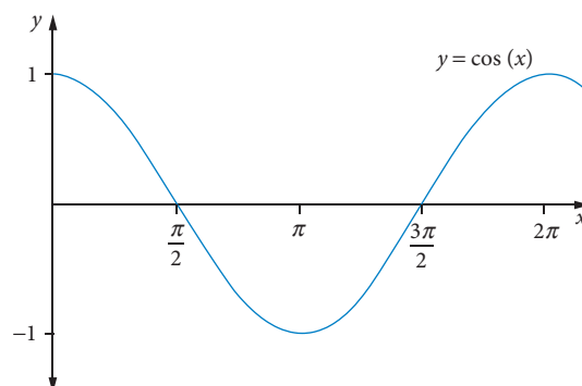
y = \cos(x) has period 2\pi and amplitude 1
