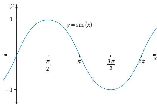
y = \sin(x) has period 2\pi and amplitude 1
