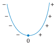
local minimum turning point
