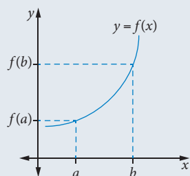
When f(x) is strictly increasing f(a) < f(b) .
