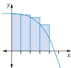
Using left rectangles
