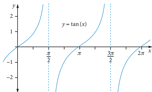
y = \tan(x) has period \pi and no amplitude
