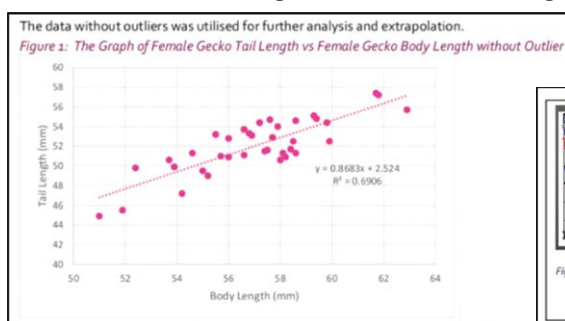
Student sample taken from the 2022 Specialist Mathematics subject report
