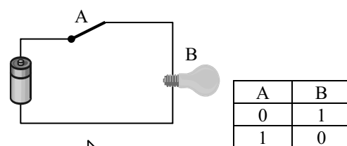
Fig 10.36 NOT gate. When switch A is up (0) the globe burns (1). When switch A is down (1) the globe does not burn (0).
