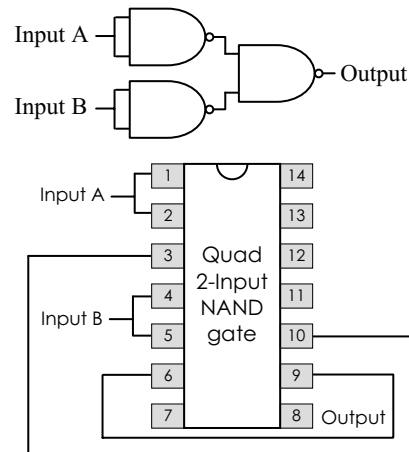
Fig 10.45 OR gate produced using 3 NAND gates.
