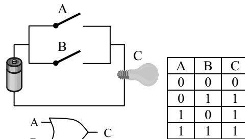
Fig 10.35 OR gate. Either A or B must be 1 for the light to burn.
