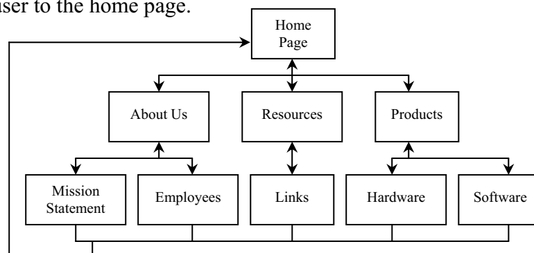
Fig 3.26 Hierarchical navigation between screens is common for web sites.
