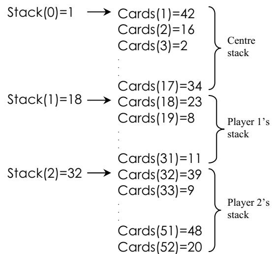
Fig 4.46 Sample data for "snap".
