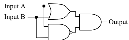
Fig 10.46 XOR gate produced using 3 different gates.
