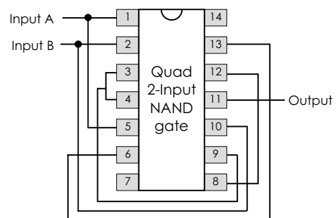
Fig 10.50 XOR gate created using an IC containing 4 NAND gates.
