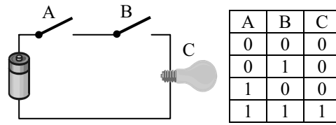
Fig 10.33 AND gate. Both A and B must be 1 for the light to burn.
