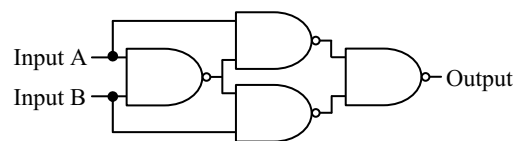
Fig 10.49 XOR gate using only 4 NAND gates.
