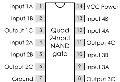
Fig 10.41 74HC series CMOS NAND integrated circuit. Contains 4 NAND gates.
