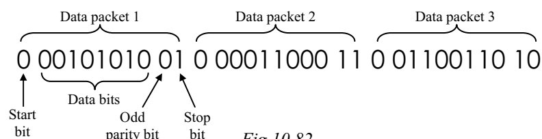
Fig 10.82 Data stream for a typical PS2 mouse transmission.
