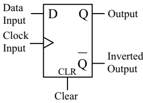
Fig 10.74 D Flip-flop with clear
