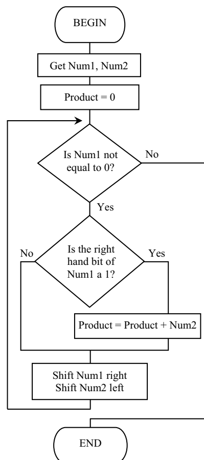
Fig 10.27 Algorithm describing binary multiplication using shifts and adds.
