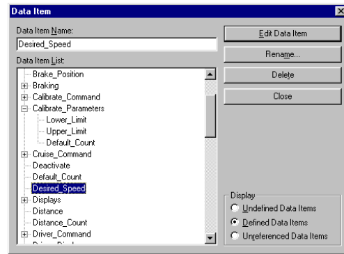
Fig 3.20 Data dictionary screen from the Axiomsys CASE tool.
