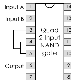
Fig 10.43 AND gate produced using 2 NAND gates.
