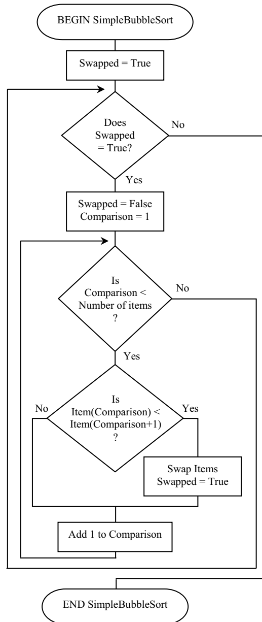
Fig 4.15 Flowchart for a simple bubble sort.
