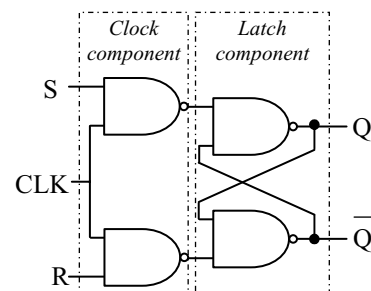
Fig 10.67 Clocked RS-NAND latch circuit.
