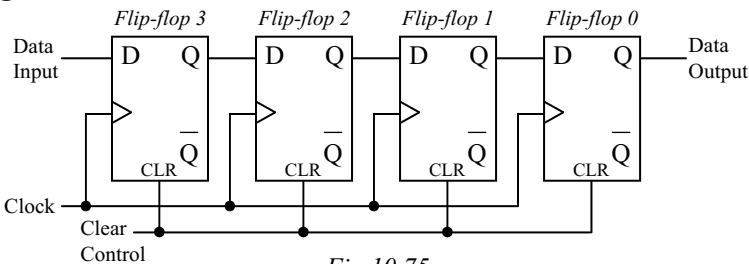
Fig 10.75 Serial in – serial out shift register
