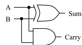
Fig 10.60 Binary half adder
