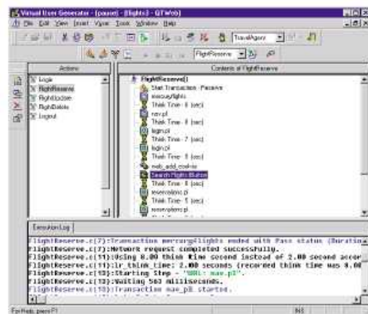
Fig 6.6 Sample screens from Mercury Interactive's LoadRunner product.
