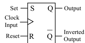
RS Flip-flop
