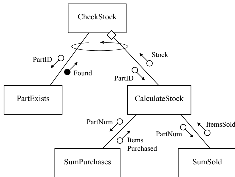
Fig 3.13 CheckStock structure chart.
