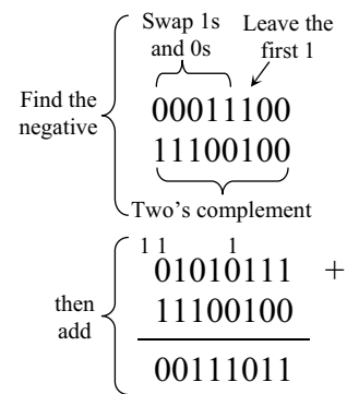
Fig 10.25 Subtraction is performed by adding the negative.
