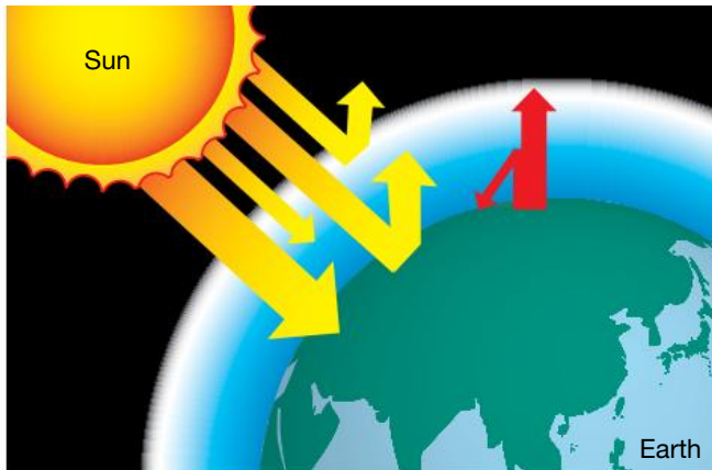
Greenhouse effect
