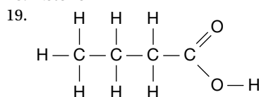
butanoic acid
