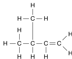
3-methylbut-1-ene
