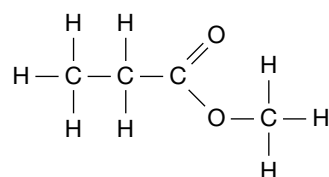
methyl propanoate
