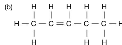
pent-2-ene
