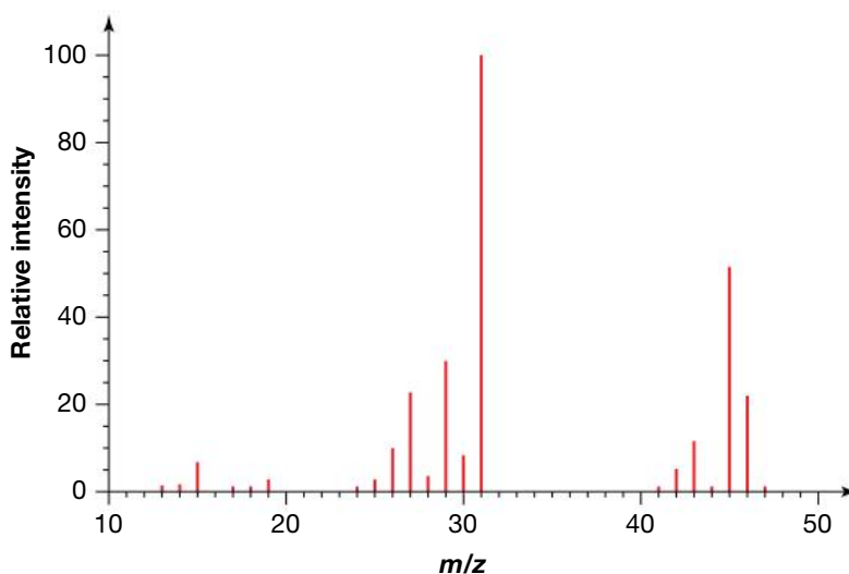
Spectrum A
