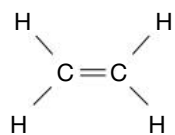
(a) ethene
