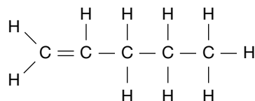
pent-1-ene
