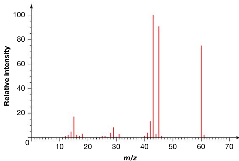
Spectrum B
