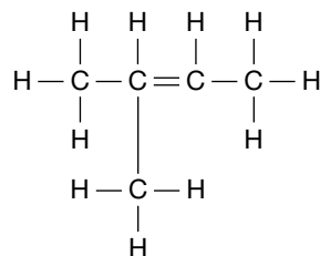
2-methylbut-2-ene
