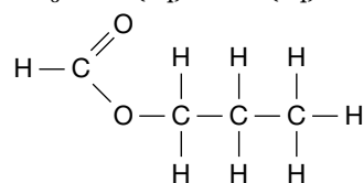
propyl methanoate
