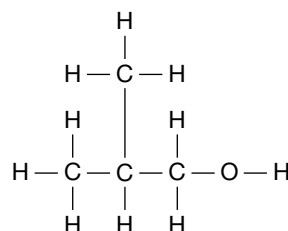
2-methylpropan-1-ol
