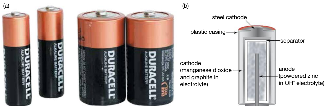
(a) Alkaline zinc/manganese dioxide cells (b) A simplified cross-section of an alkaline zinc/manganese dioxide cell
