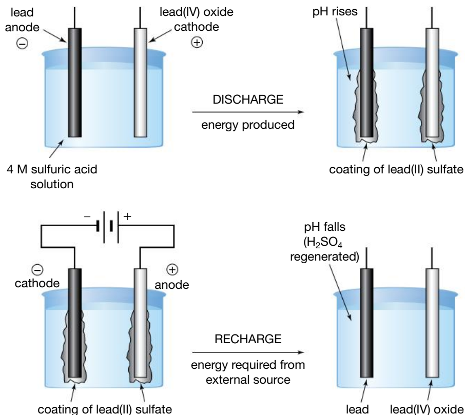
Discharge/recharge effect on electrodes
