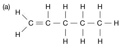
pent-1-ene
