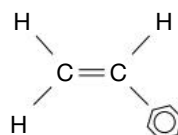
(c) styrene
