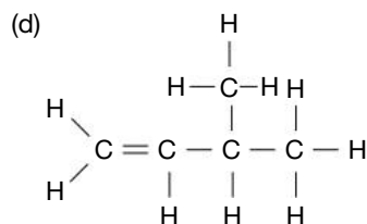
3-methylbut-1-ene
