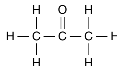
propanone
