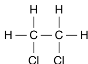
1,2-dichloroethane, \text{CH}_2\text{ClCH}_2\text{Cl}
