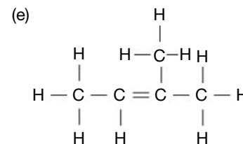
2-methylbut-2-ene
