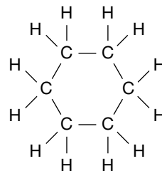
cyclohexane
