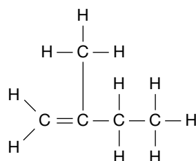
2-methylbut-1-ene
