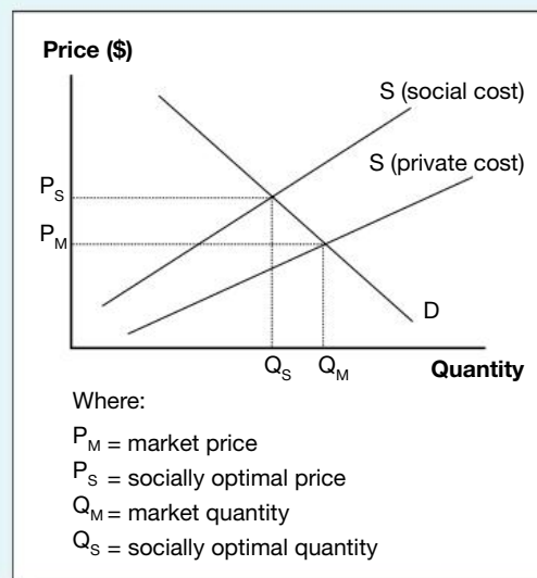
Figure 8.8 – Market failure
