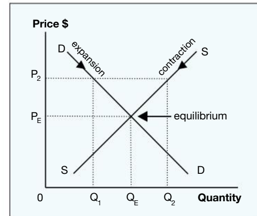
Figure 8.3 – Excess supply
