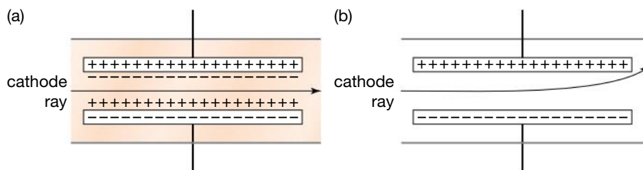
Cathode ray path (a) at high and (b) low gas pressure. At higher pressures a sheath of ionised gas shields the cathode rays from the effects of the applied electric field.
