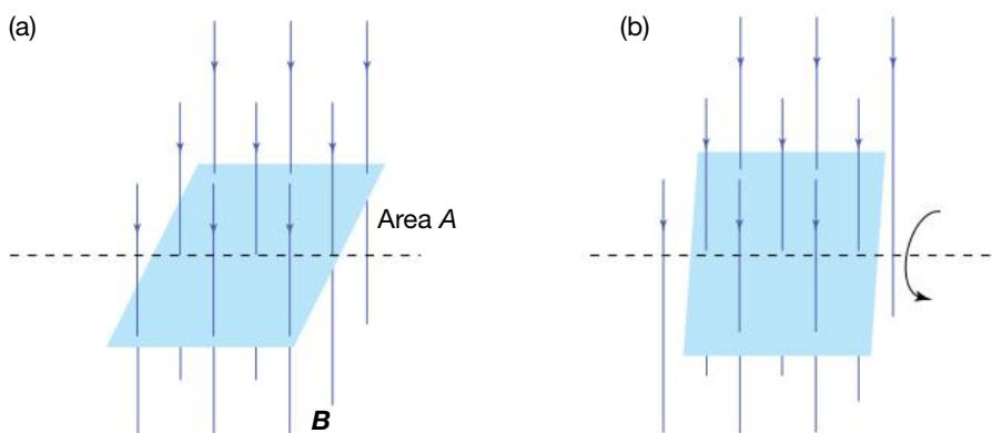
Magnetic flux is the amount of magnetic field passing through an area. In (a) it is the maximum BA ; in (b) the value is less, as fewer field lines pass through the coil.
