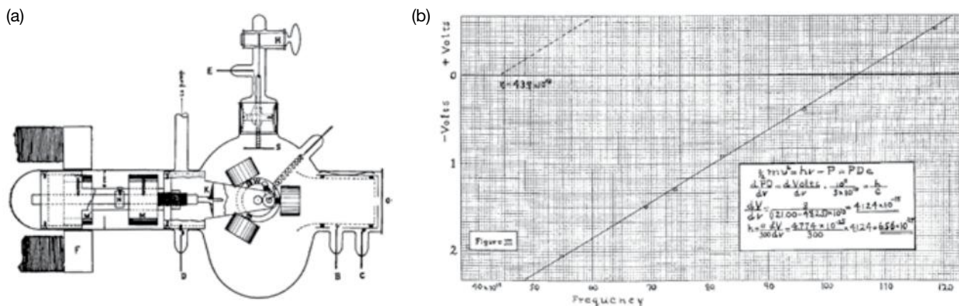
(a) Millikan's 'machine shop in a glass tube', and (b) his first published results
