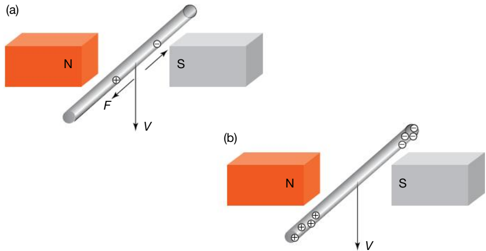
The magnetic field forces electrons to the far end of the falling rod.
