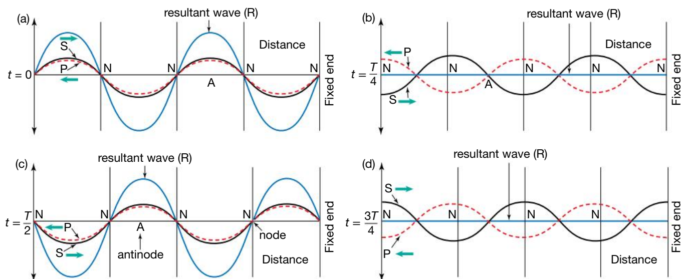
The formation of a standing wave
