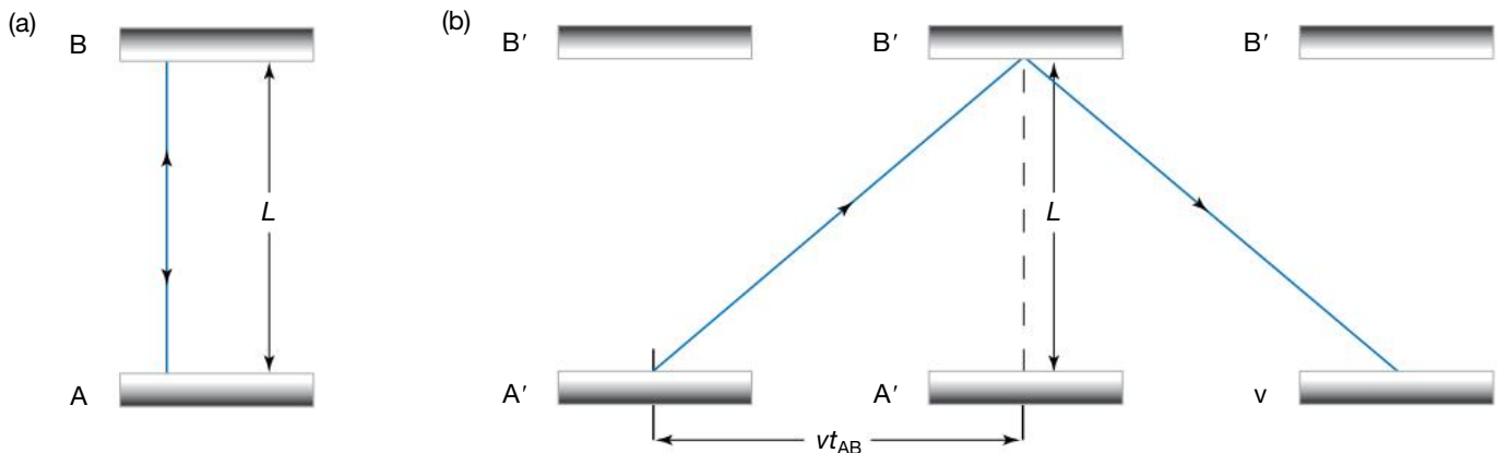
A light clock (a) at rest relative to the observer, and (b) in motion relative to the observer
