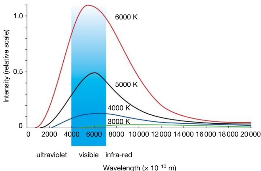
Thermal radiation for an ideal black body
