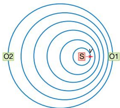
(b) Source moving to the right
