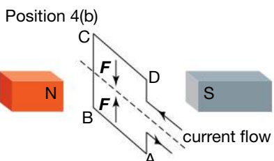
Force on a coil in a DC motor
