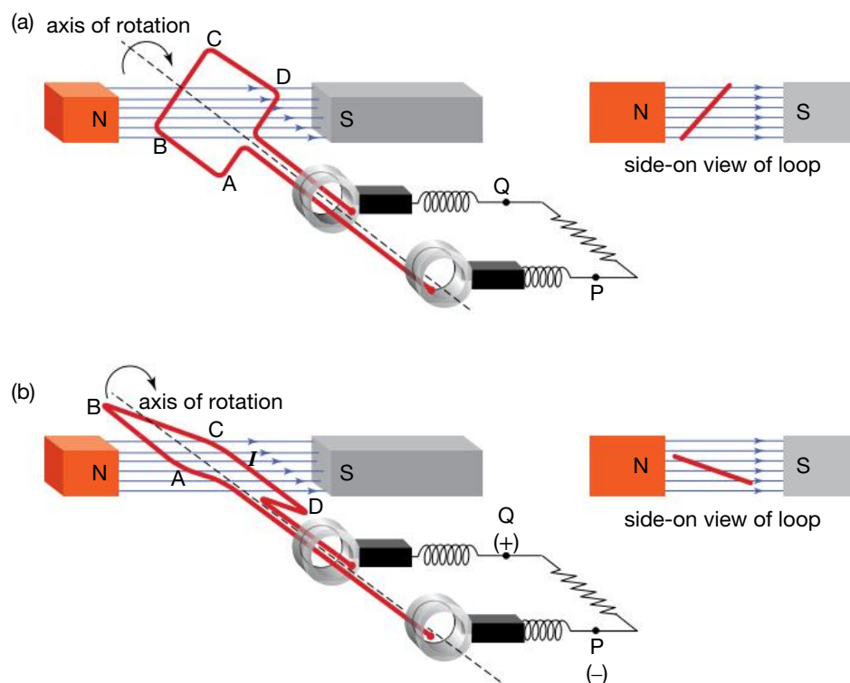
Direction of current flow as loop passes through the horizontal position
