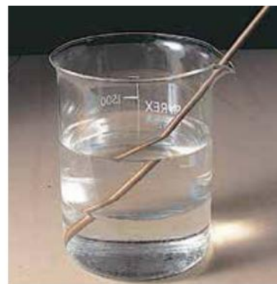
An example of refraction
