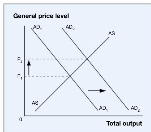
Figure 9.3 – Demand-pull inflation
