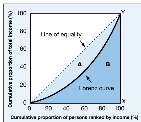
Figure 11.3 – Lorenz curve
