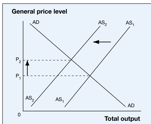
Figure 9.4 – Cost-push inflation
