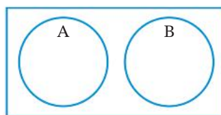
Mutually exclusive events: 'A or B' means A or B but not both
