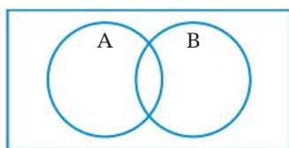
Overlapping events: 'A or B' means A or B or both
