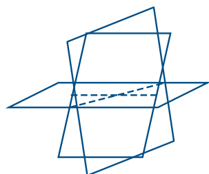
Diagram 1: Intersection at a point
