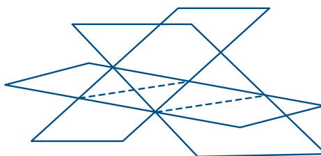
Diagram 5: No common intersection
