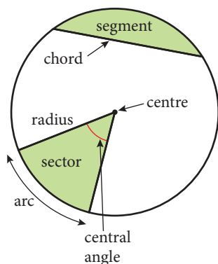
Figure 5.1 The parts of a circle
