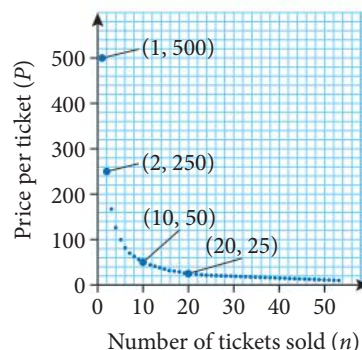
Figure 6.28 Price per ticket varies inversely with the number of tickets sold
