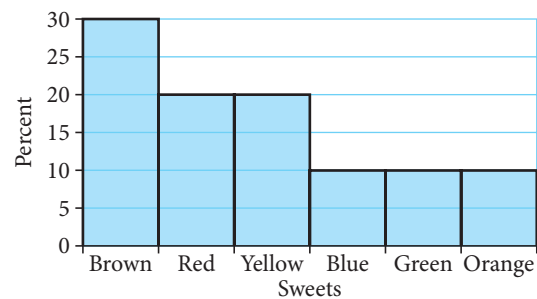
Figure 7.7 Relative frequency distribution
