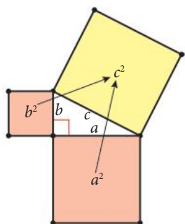
Figure 4.2 The squares formed using the base and the height of a right-angled triangle as side lengths fit perfectly in the square formed by using the hypotenuse as a side length
