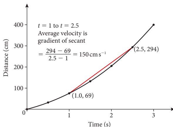
Figure 9.9 Average velocity from t = 1 to t = 2.5
