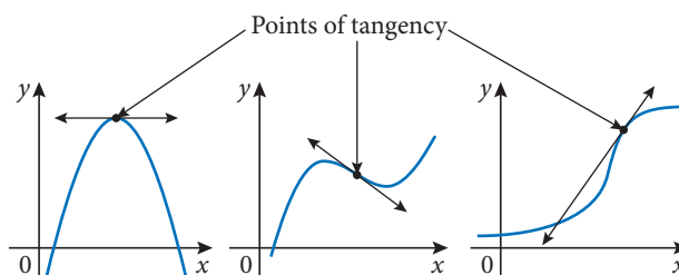
Figure 9.14 Different configurations of tangent lines
