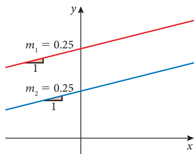
Figure 2.3 Two lines for which the gradients, m_1 and m_2 are equal. The lines are parallel
