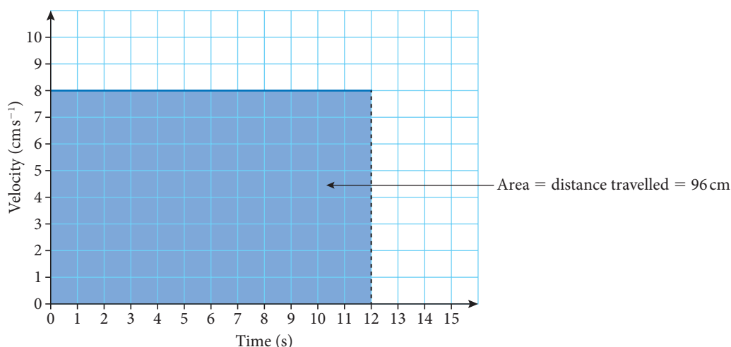
Figure 11.9 Area under the function
