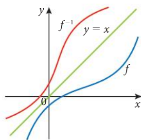
Figure 2.22 The graphs of f and f^{-1} are symmetrical about the line y = x
