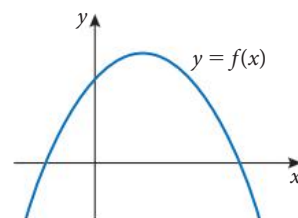
Figure 11.10 Graph of f(x) = -x^2 + 2x + 3
