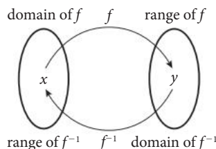
Figure 2.20 A mapping diagram for a pair of inverse functions
