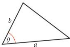
Figure 4.16 Area of triangle with two sides and the included angle
