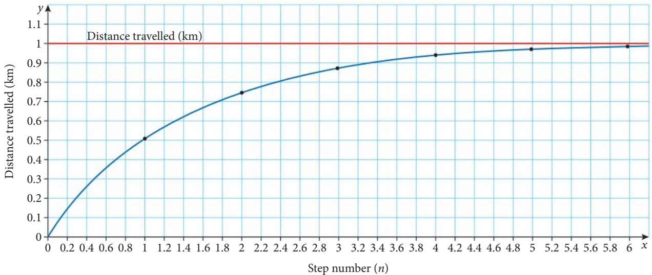
Figure 9.2 D_n = 1 - \frac{1}{2^n} and D = 1
