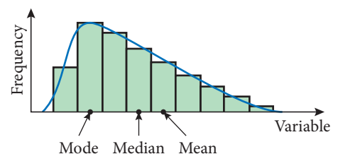
Figure 7.20 Positively skewed distribution
