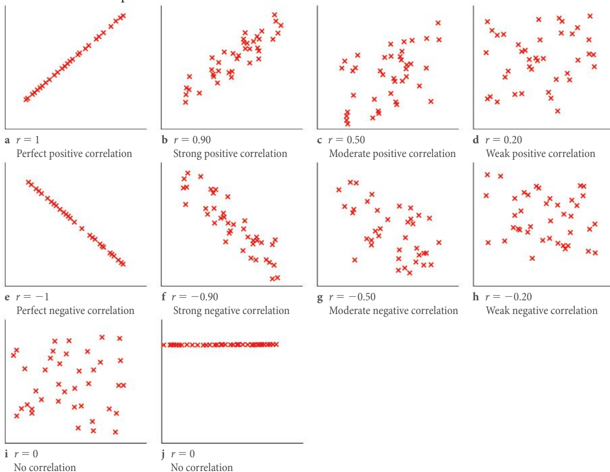
Figure 14.13 Examples of r
