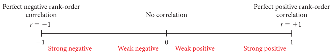
Figure 14.17 Interpretation of Spearman's r_s .
