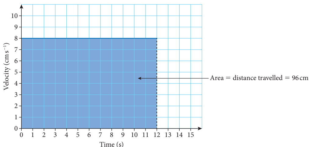
Figure 11.1 The shaded area represents the distance travelled in 12 seconds at 8 \text{ cm s}^{-1}
