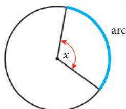
Figure 5.2 An arc and its central angle
