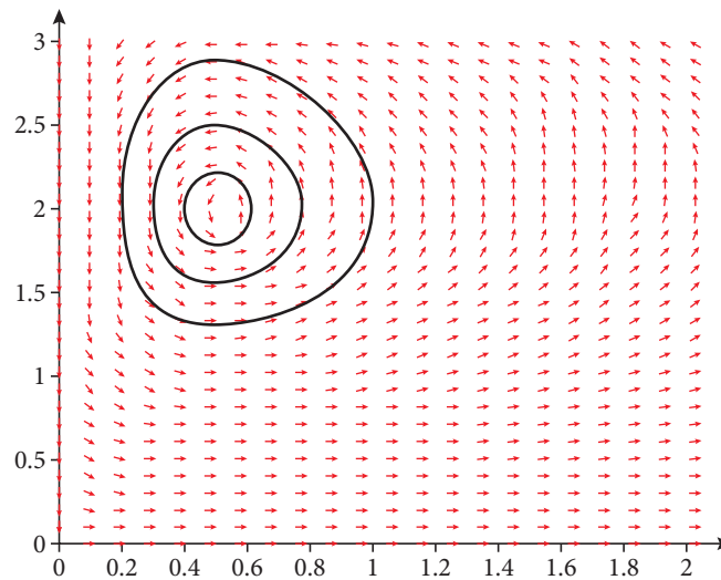
Figure 2 A phase space diagram. Number of prey (in units of 1000) on the x-axis, number of predators on the y-axis
