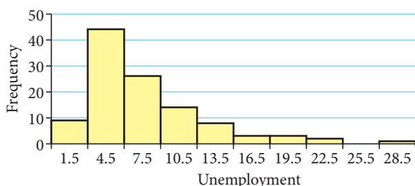
Figure 7.9 Histogram for unemployment data using midpoints
