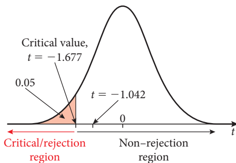
Figure 13.10 Hypothesis testing using critical values
