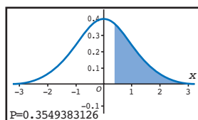
Figure 13.13 Running the usual 2-sample t -test
