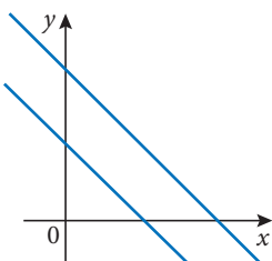
Figure 2.5 Possible relationship between two lines in a coordinate plane
