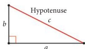
Figure 4.1 a^2 + b^2 = c^2
