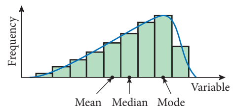
Figure 7.21 Negatively skewed distribution
