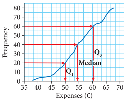
Figure 7.26 Ogive for expense data
