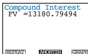
Figure 3.10 Using a GDC to calculate compound interest
