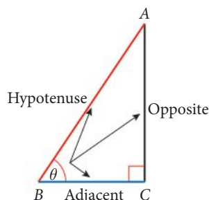
Figure 4.10 The sides of a triangle can be labelled as adjacent, opposite and hypotenuse
