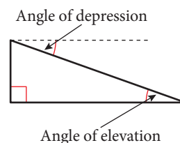
Figure 4.18 Angle of depression and angle of elevation
