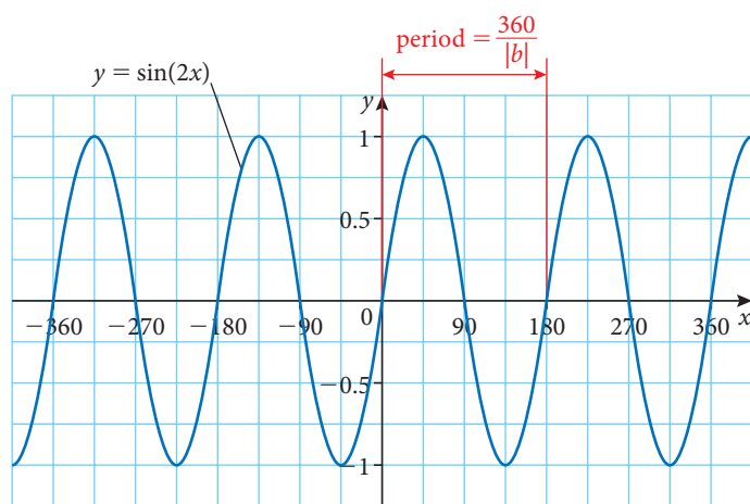
Figure 6.31 Relationship between period and b
