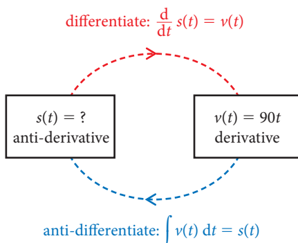
Figure 11.4 For what function is v(t) = 90t the derivative?
