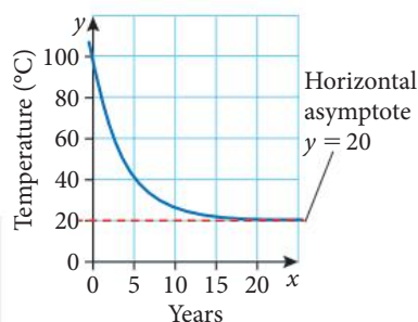
Figure 6.26 Horizontal asymptote at y = 20
