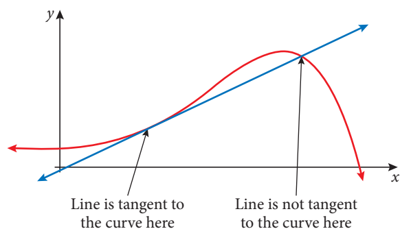
Figure 9.13 Graphical illustration of a tangent line
