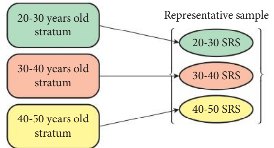
Figure 7.5 Stratified random sampling
