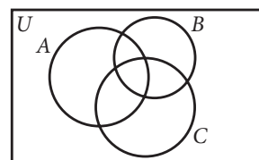
Figure 8.13 Venn diagram for question 1 (b)
