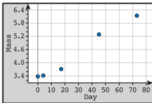
Figure 6.39 Mass versus days since birth for a young child
