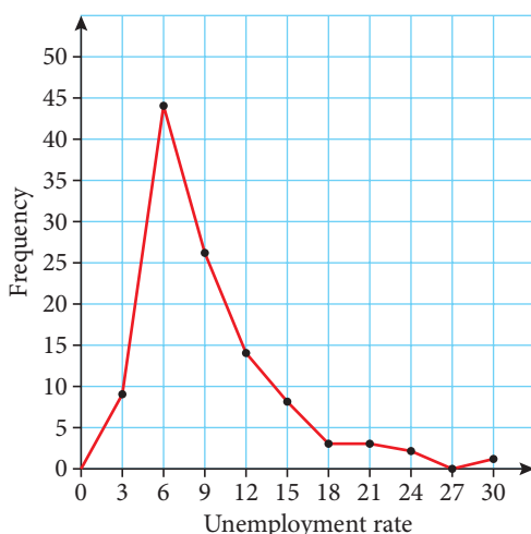
Figure 7.12 Frequency graph for unemployment data
