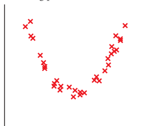
b r = -0.02 No correlation?
