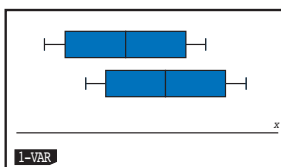
Figure 7.29 New box plot shifted to the right by 5 units
