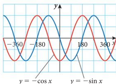
Figure 6.34 When a < 0 , the graphs of sine and cosine are reflected across the x axis. This causes a change in behaviour around x = 0 that is important for modelling
