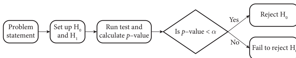
Figure 13.5 Steps for conducting a hypothesis test
