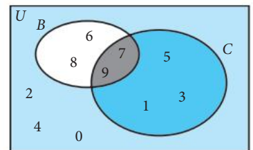
Figure 8.9 Intersection of events
