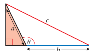
Figure 4.30 Interpretation of the cosine rule when \theta > 90^\circ
