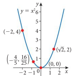
Figure 2.1 Graph of the solution set of the equation y = x^2
