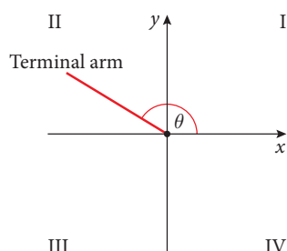
Figure 4.21 Angles larger than 90^\circ
