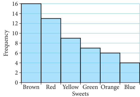
Figure 7.6 A bar graph of colours of sweets
