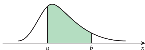
Figure 12.14 Shaded area gives the probability P(a \leq x \leq b)
