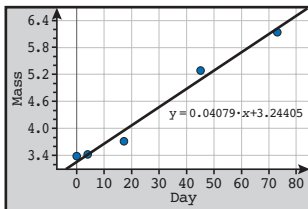
Figure 6.40 Linear model for mass in terms of days after birth
