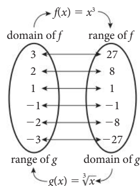
Figure 2.19 A mapping diagram for the cubing and cube root functions
