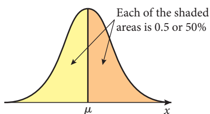
Figure 12.18 The curve is symmetric about the mean
