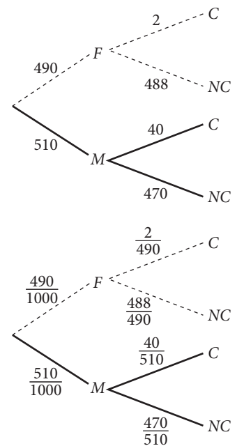
Figure 8.12 Tree diagrams for colour blindness
