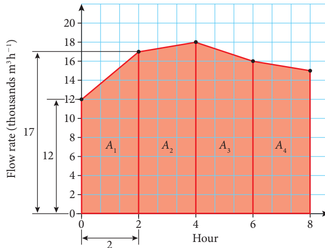
Figure 11.19 Using trapeziums to calculate the area under a curve based on data
