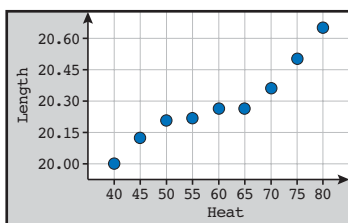
Figure 14.15 Scatter diagram for Example 14.3 (a)
