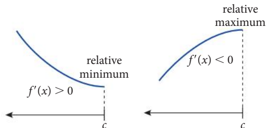
Figure 10.4 Right-hand endpoints of domain (upper bounds)
