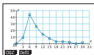
Figure 7.14 GDC frequency graph
