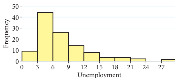
Figure 7.8 Histogram of the unemployment data
