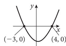
Figure 9.17 The derivative function is concave up
