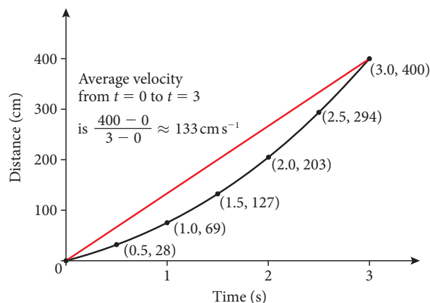
Figure 9.7 Distance–time graph; average velocity from t = 0 to t = 3
