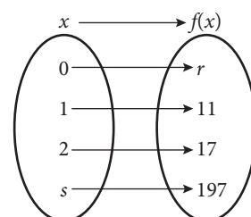
Figure 2.25 Mapping diagram for question 6
