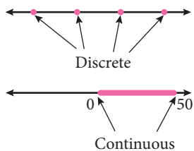
Figure 12.1 Discrete and continuous variables
