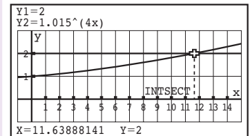
Figure 3.5 GDC screen for the solution to Example 3.13
