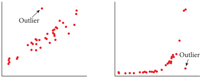
Figure 14.8 Outliers are a departure from the predominant pattern
