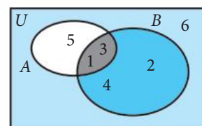
Figure 8.2 Sample space and events of rolling a dice
