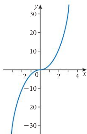
Figure 2.21 Graph of f(x) = x^3 which is increasing as x goes from -\infty to \infty
