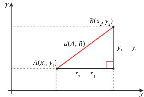
Figure 4.4 The line segment [AB] forms the hypotenuse of a right-angled triangle
