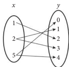
Figure 2.9 Mapping for a set of x values to a set of y values
