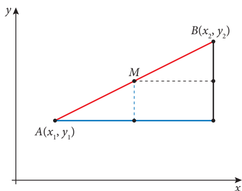
Figure 4.6 The midpoint of a line segment
