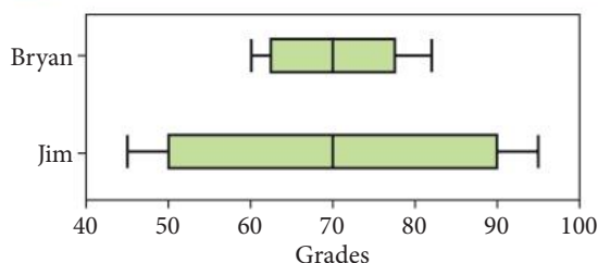
Figure 7.24 Box plot of grades
