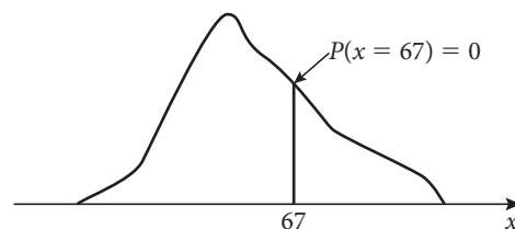
Figure 12.16 Probability of a single value is zero
