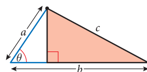
Figure 4.29 Interpretation of the cosine rule when \theta < 90^\circ
