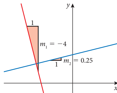
Figure 2.4 Two lines for which the product of the gradients, m_1 and m_2 is -1 are perpendicular
