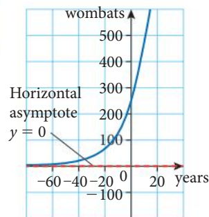
Figure 6.25 Horizontal asymptote at y = 0
