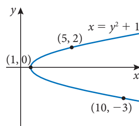
Figure 2.12 The graph of x = y^2 + 1
