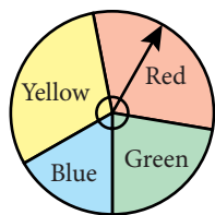
Figure 8.8 Spinner in question 2
