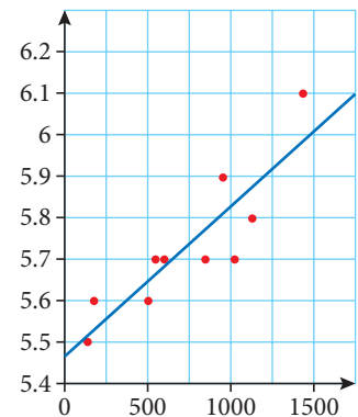
Figure 14.11 The data shows a strong, positive, linear correlation
