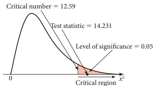
Figure 13.15 Test statistics in the critical region – reject H_0
