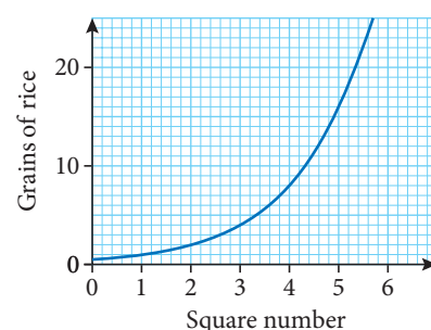
Figure 6.19 Zooming in on the graph
