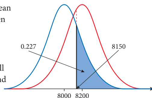
Figure 13.4 Area for type II error
