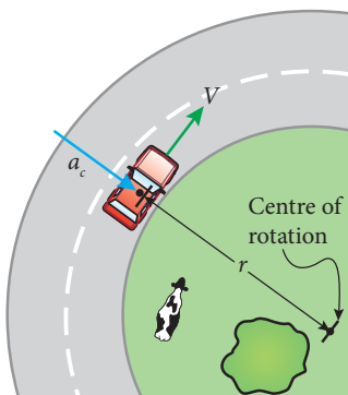
Figure 10.8 When a car is travelling through a turn, the momentum of the car is trying to carry the car in a direction tangent to the curve of the road. The car's tyres must generate a force normal to the curve of the road in order to steer the car around the curve
