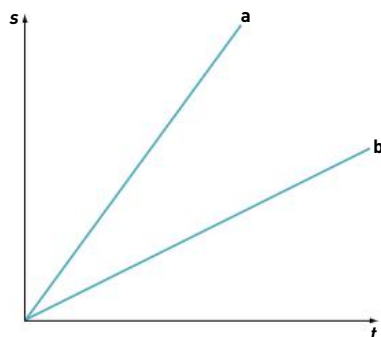
Figure 7.15 Speed–time graphs showing a (a) steep gradient, indicating high acceleration, and (b) gentle gradient, indicating lower acceleration.
