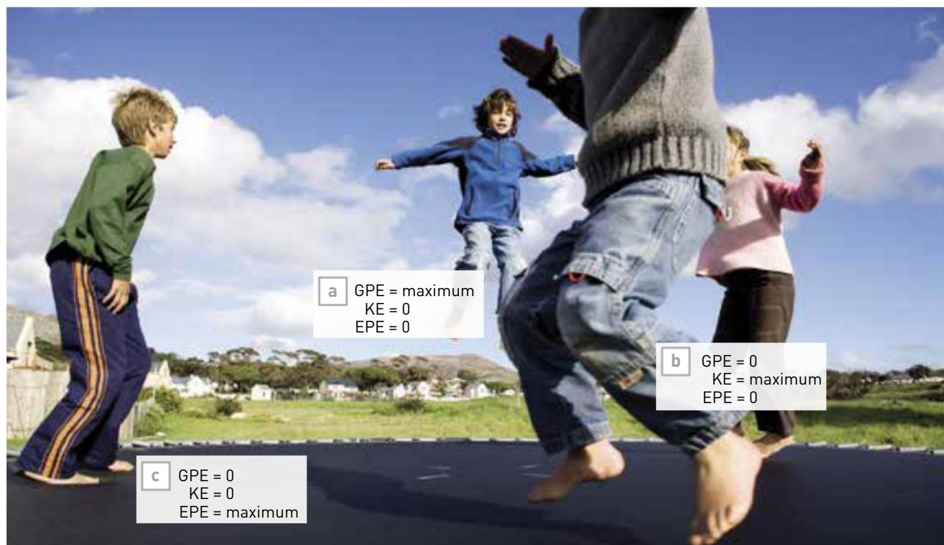
Figure 7.39 Although the individual energy quantities vary between the highest point (a), through position (b) to the lowest position (c), the total energy of the 'system' remains constant.
