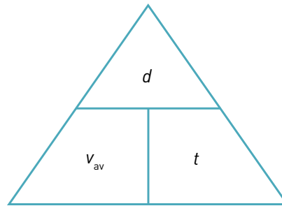
Figure 7.8 The average velocity triangle. Cover the quantity you want to calculate and the other two quantities will form the formula.
