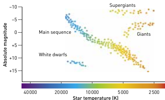
Figure 6.4 A Hertzsprung–Russell diagram.
