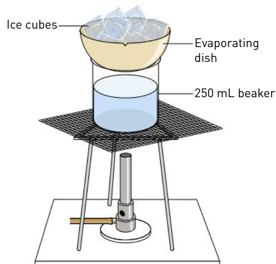
Figure 8.15 Experimental set-up.
