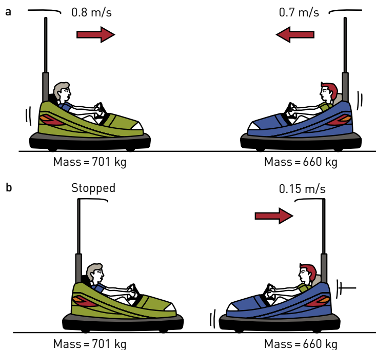
Figure 7.35 (a) Before the collision. (b) After the collision.
