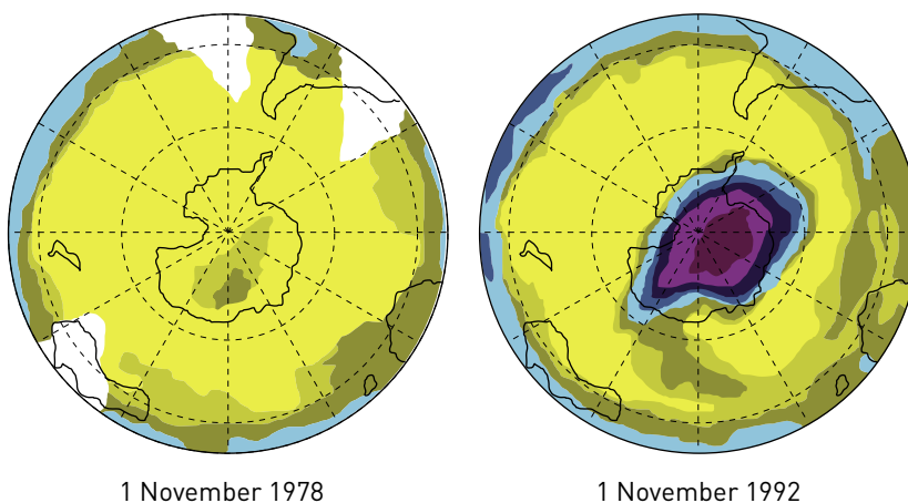
Figure 4.28 Ozone levels reduce over the southern hemisphere every year. The darker colours show where the 'hole' in the ozone layer has grown.
