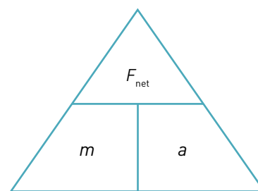
Figure 7.26 The net force equation can be written as a triangle. Cover the quantity you want to calculate and the other two quantities will form the formula.
