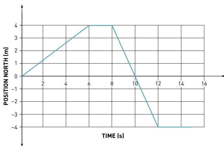
Figure 7.1 This position–time graph shows the position of a person walking north from the starting point for 6 seconds, stopping for 2 seconds and then walking south for 4 seconds. Their final position was 4 metres south of the starting point.
