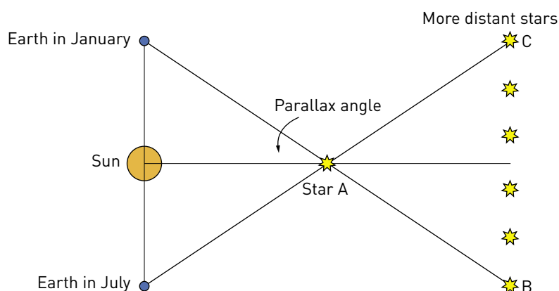
Figure 6.5 Measuring the distance to stars using stellar parallax. In January, star A, a close star, is in line with a more distant star, star B, but in July it is in line with star C. By measuring the parallax angle and knowing the radius of the Earth's orbit, the distance to star A can be calculated.
