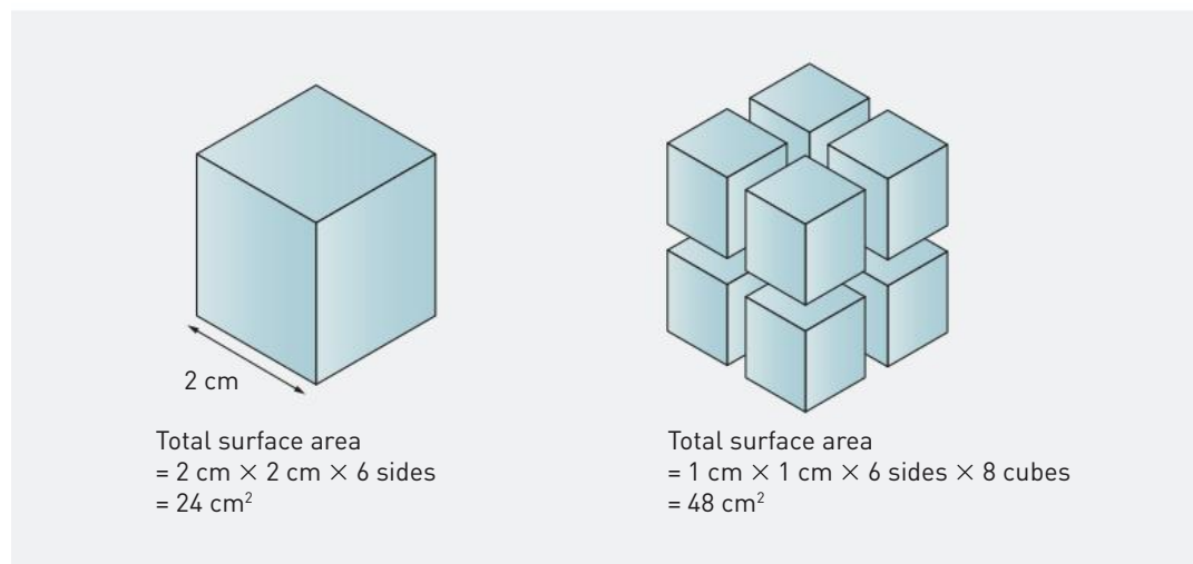
Figure 4.20 Many small particles have a larger surface area than a single large particle of the same volume.
