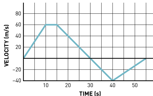
Figure 7.9 This velocity–time graph shows an object with changing velocity. The object increases its velocity from 0 m/s to 60 m/s in the first 10 seconds. It then travels at a constant 60 m/s for 5 seconds before slowing down. At 30 seconds, it has stopped and then starts travelling in the opposite (negative) direction before eventually slowing to a stop. The area under the graph describes the displacement as 1050 metres in the positive direction and 500 metres in the negative direction. The total displacement will be 250 metres in the positive direction.
