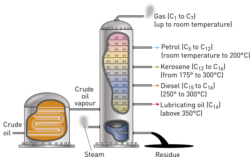
Figure 4.7 As the crude oil is slowly heated, vapour (gases) form. As the vapour rises, it cools. When the vapour reaches the height where the temperature is equal to the fraction's boiling point, it condenses into a liquid.
