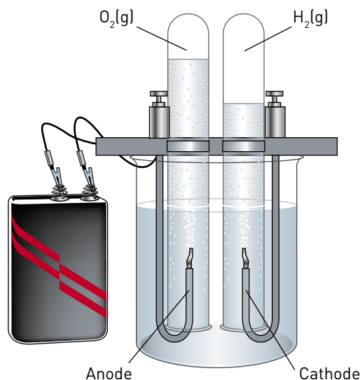
Figure 4.1 Electrolysis equipment. At the anode, water is being broken down into oxygen gas and hydrogen ions. At the cathode, hydrogen gas is being produced from hydrogen ions and electrons.
