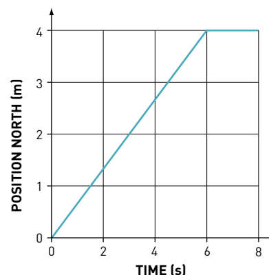
Figure 7.6 The speed of the object in this position–time graph can be calculated by determining the gradient of the graph. Gradient = change in position ÷ change in time = rise ÷ run = 4 \text{ m} \div 6 \text{ s} = 0.67 \text{ m/s} .
