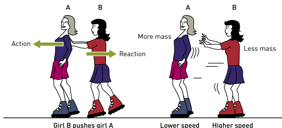
Figure 7.30 Different masses have different accelerations and reach different speeds even though the forces shown by the arrows are equal in size.
