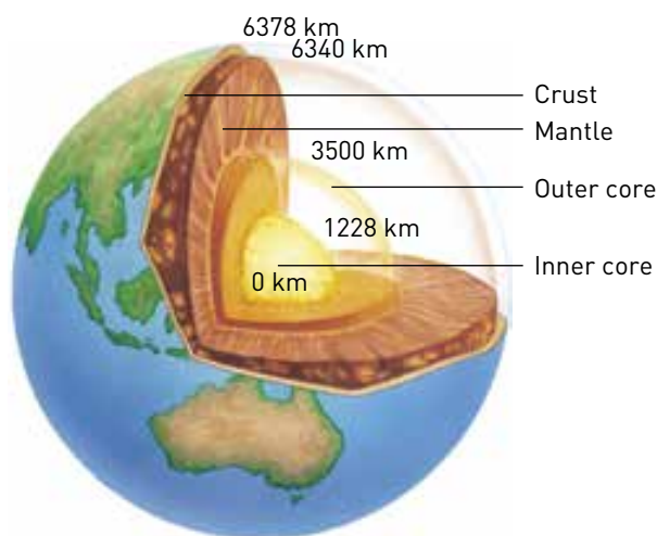
Figure 5.1 The Earth is made up of layers.
