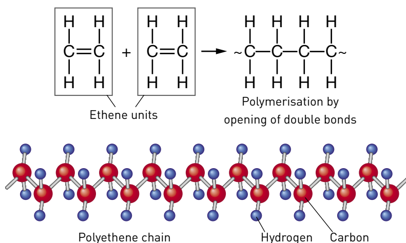
Figure 4.13 The formation of polyethene from ethene molecules.
