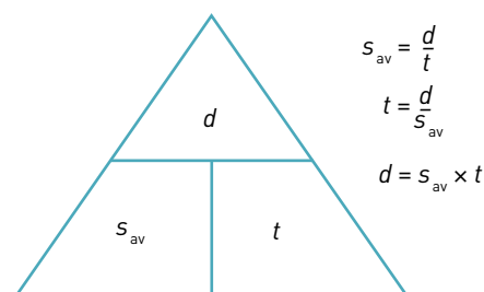
Figure 7.5 The average speed triangle is used to work out the formula for average speed. Cover the quantity you want to calculate with your finger and the other two quantities will form the formula.
