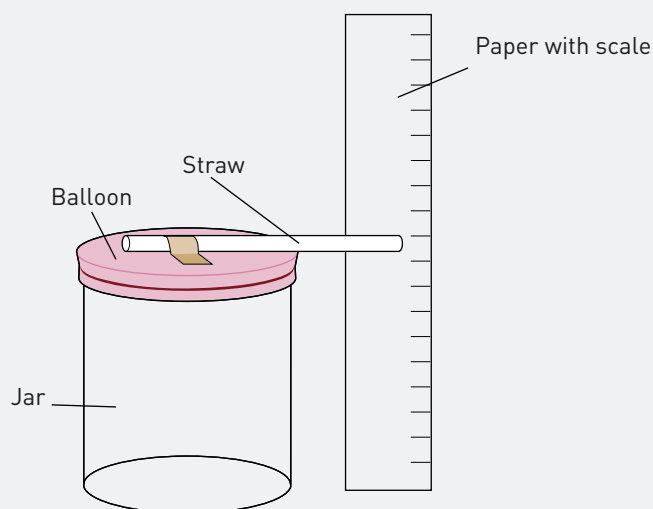
Figure 8.16 Experimental set-up.
