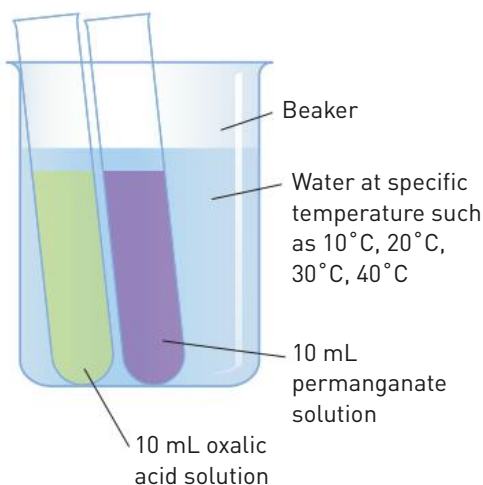
Figure 8.14 A water bath can be used to control the temperature of the solutions.
