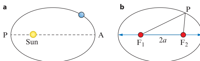
Figure 17.7: a The orbits of planets are elliptical. b The ellipse has two special points on its long axis, called the foci. The sum of the distances of any point on the ellipse from each of the foci is a constant.
