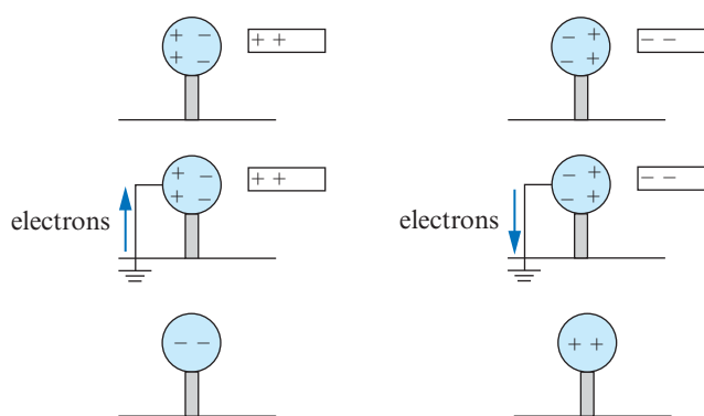
Figure 18.3: Charging a sphere by induction.
