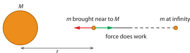
Figure 17.11: Work is done to bring the small mass from infinity to a given position near the big mass. The red arrow is the force of attraction between the two masses. We are interested in the work done by the force represented by the green arrow, i.e. the work done by the external agent. This work is negative and is stored as potential energy. The work done is independent of the actual path followed.
