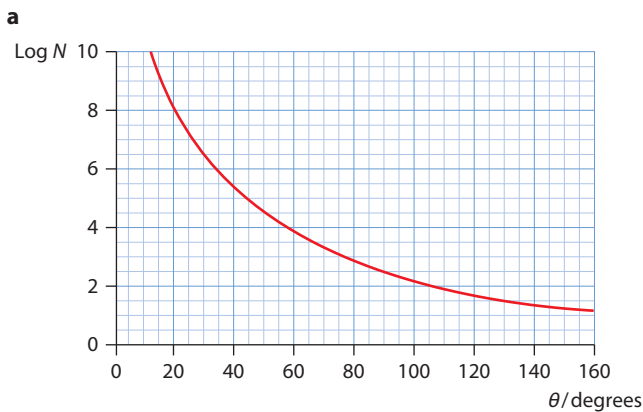
Figure 23.9: a The logarithm of the number of alpha particles scattered at some angle \theta as a function of \theta . b The logarithm of the number of alpha particles scattered at an angle of 60^\circ as a function of the alpha particle energy. The dotted curve is based on Rutherford scattering. The blue curve is the observed curve. We see deviations when the energy exceeds about 28 MeV. The energy at which deviations start may be used to estimate the nuclear radius.
