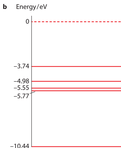
Figure 21.4: Energy level diagrams according to Bohr: a for hydrogen, and b for mercury.
