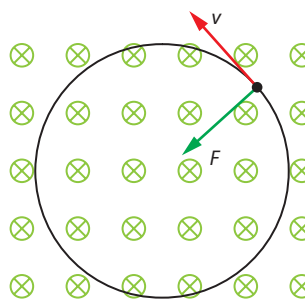
Figure 19.15: A charge in a magnetic field moves in a circle.
