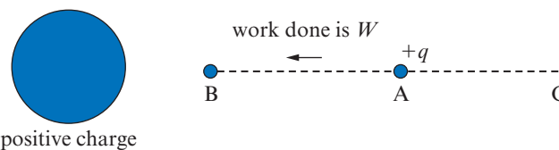
Figure 11.1: The potential difference between points A and B is the work done to move the charge from A to B divided by q . If the charge q is released at A it will accelerate to the right, gaining kinetic energy.
