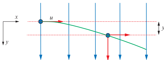
Figure 19.5: The path of the particle is parabolic.
