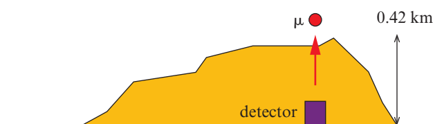
Figure 6.18: From the point of view of an observer on the muon the mountain is much shorter.
