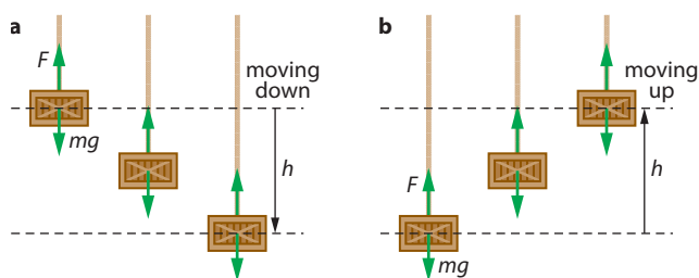
Figure 3.8: Lowering and raising an object at constant speed using a rope.
