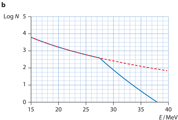
Figure 23.9: a The logarithm of the number of alpha particles scattered at some angle \theta as a function of \theta . b The logarithm of the number of alpha particles scattered at an angle of 60^\circ as a function of the alpha particle energy. The dotted curve is based on Rutherford scattering. The blue curve is the observed curve. We see deviations when the energy exceeds about 28 MeV. The energy at which deviations start may be used to estimate the nuclear radius.
