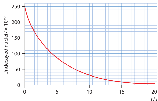
Figure 23.17: Radioactive decay follows an exponential decay law.
