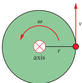
Figure 5.2: Linear and angular velocities.
