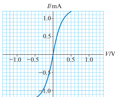
Figure 11.5: The current–potential difference graph for a filament lamp; the resistance increases as the voltage increases.
