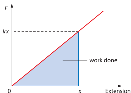
Figure 3.10: The force F stretches the spring. The force is proportional to extension according to Hooke's law.
