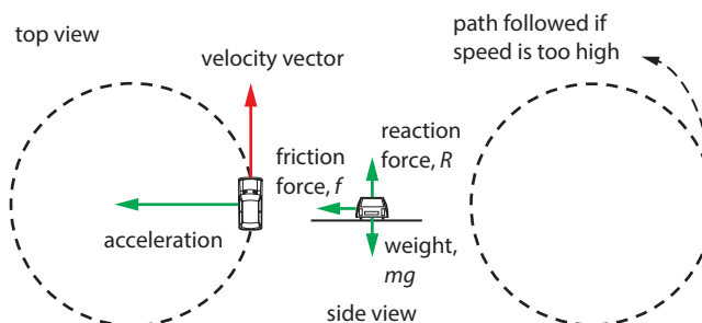
Figure 2.62: A car will skid outward (i.e., will cover a circle of larger radius) if the friction force is not large enough.
