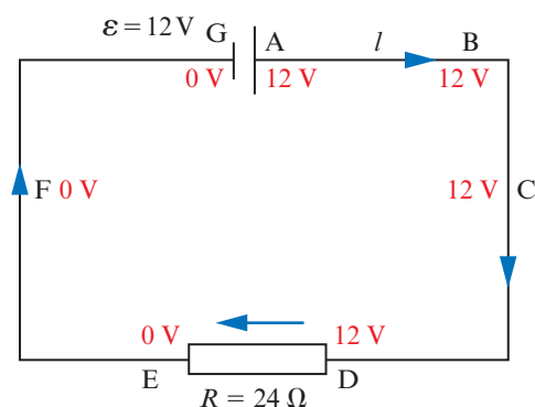
Figure 11.18: A simple one-loop circuit with one cell with negligible internal resistance and one resistor.
