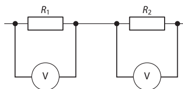
Figure 11.47: A voltmeter is connected in parallel to the device we want to measure the potential difference across.
