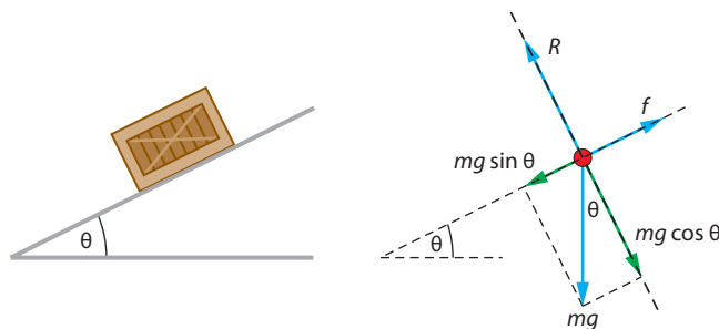
Figure 2.42: A block at rest on an inclined plane.
