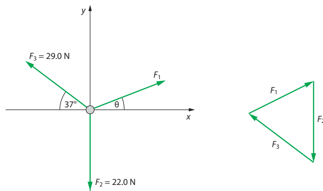
Figure 2.36: Force diagram of three forces in equilibrium pulling a common point. Notice that the three vectors representing the three forces form a triangle.
