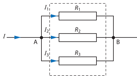
Figure 11.23: Three resistors connected in parallel.
