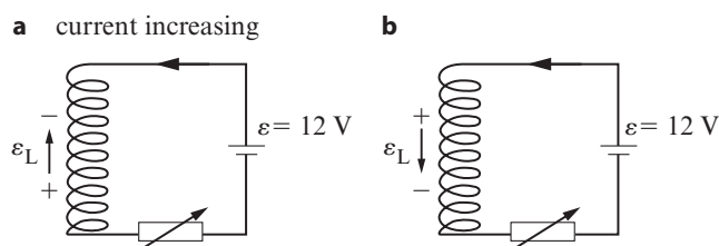
Figure 20.18: When the current is a increasing or b decreasing there is an induced emf in the coil.
