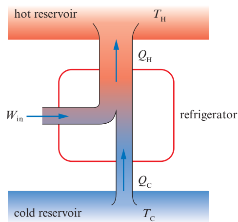
Figure 10.23: In a refrigerator mechanical work is used to extract heat from a cold reservoir and deposit it in the hot reservoir.
