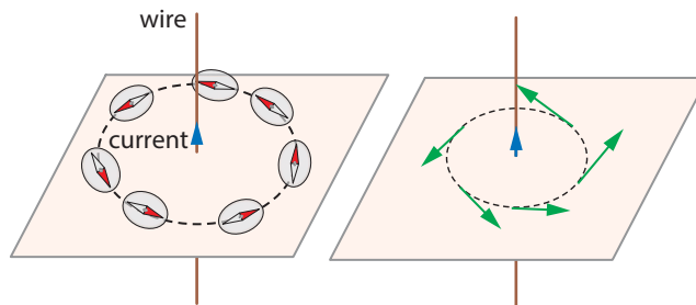
Figure 18.27: Magnetic field around a straight wire.
