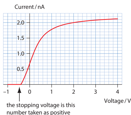
Figure 22.2: When the collecting plate is connected to the negative terminal of the power supply, there is a voltage at which the current becomes zero (Vs). This is 0.4 V in this example.
