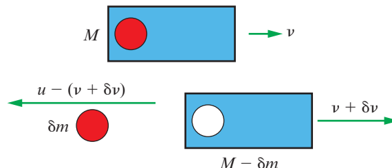
Figure 4.14: Deriving the rocket equation: The velocities are all relative to an observer 'at rest on the ground'.
