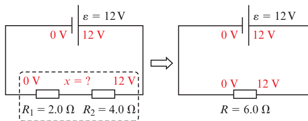
Figure 11.19: Finding the total resistance of the circuit.
