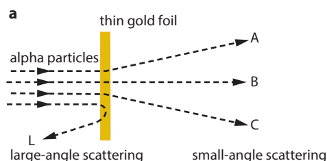
Figure 21.1: a The majority of alpha particles are slightly deflected by the gold foil. Very occasionally, large-angle scatterings take place. b The alpha particles are detected by the sparks of light they create when they hit a zinc sulfide screen in the microscope.
