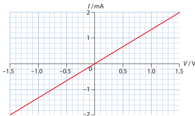
Figure 11.4: The current–potential difference graph for a material that obeys Ohm's law.
