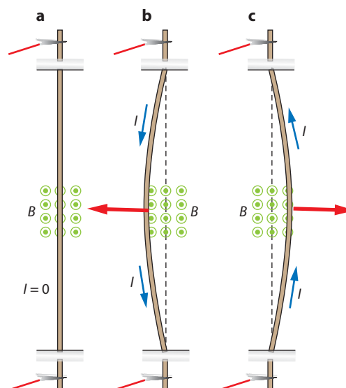
Figure 18.41: The magnetic force on a current-carrying wire.
