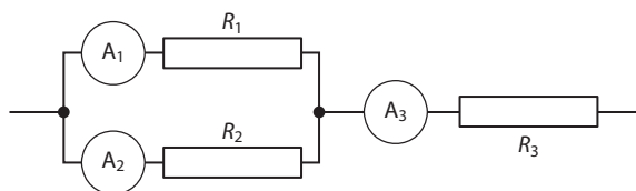
Figure 11.46: An ammeter measures the current in the resistor connected in series to it.
