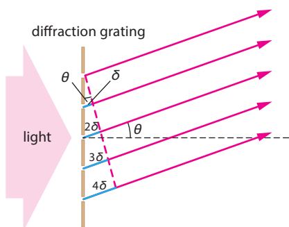
Figure 14.58: The path difference between any two rays is an integral multiple of the smallest path difference \delta between the top two rays. The red dashed line is normal to the rays, which makes the angle between this line and the grating \theta .
