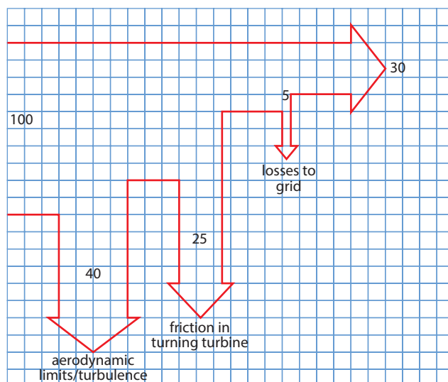
Figure 3.33: Sankey diagram for a wind turbine.
