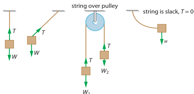
Figure 2.4: More examples of tension forces.
