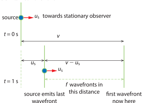
Figure 16.5: Determining the Doppler frequency.
