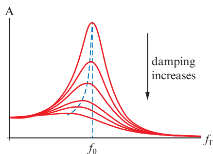
Figure 15.16: Graph showing the variation with driving frequency of the amplitude of oscillations when the system is driven by an external periodic force. For very small damping, the peak occurs at a frequency very close to the natural frequency. As the damping increases, the peak occurs at a frequency less than f_0 , as indicated by the dark dashed curve.
