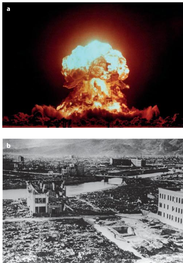
Figure 24.1: a Vast amounts of energy are released in the detonation of a nuclear weapon. b The results are catastrophic, as this photograph of Hiroshima shows.
