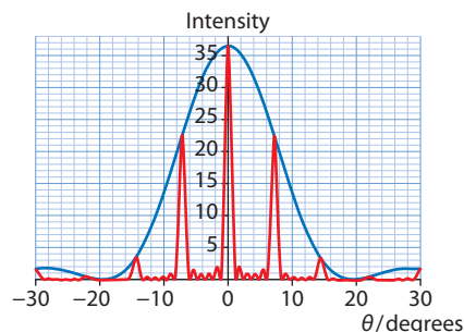
Figure 14.55: The intensity distribution for six slits. Note how the width of the maxima decreases but their position stays the same. Note also how the relative importance of the secondary maxima decreases with increasing slit number.
