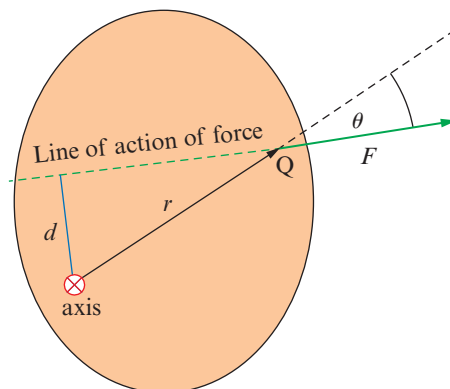
Figure 5.5: The line through the vector representing the force is called the line of action of the force. Torque is the product of the magnitude of the force times the perpendicular distance between the axis and the line of action of the force.
