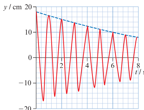
Figure 15.13: In damped oscillations the amplitude is decreasing with time exponentially.
