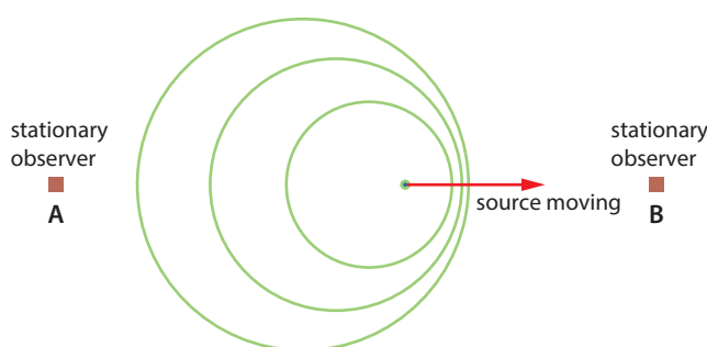
Figure 16.2: A source is moving away from a stationary observer A and is approaching the stationary observer B.
