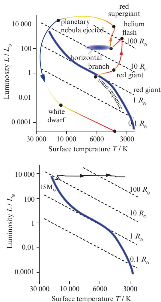
Figure 25.8: a Evolutionary path of a low mass star. This is the path of a star of one solar mass that ends up as a white dwarf, which continues to cool down, moving the star ever more to the right on the HR diagram. b This is the path of a star of 15 solar masses. It becomes a red supergiant that explodes in a supernova. After the supernova, the star becomes a neutron star, whose luminosity is too small to be plotted on the HR diagram.
