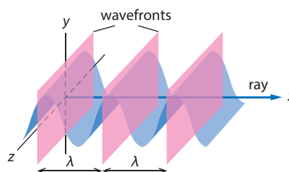
Figure 14.1: Surfaces through crests and normal to the direction of energy propagation of the wave are called wavefronts. Rays are mathematical lines perpendicular to the wavefronts and give the direction of energy transfer.
