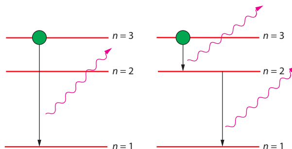
Figure 21.5: Transitions from n = 3 in hydrogen.
