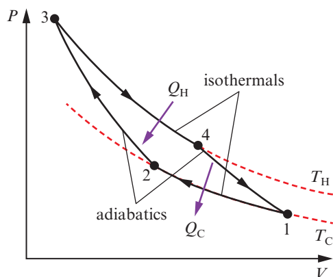
Figure 10.24: The Carnot cycle consists of two isothermals and two adiabatics.
