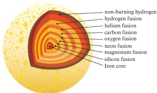
Figure 25.13: The central core of fully evolved massive star consists of iron with layers of successively lighter elements surrounding it.
