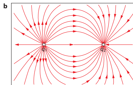
Figure 18.7: Field lines for a two equal positive charges and b two equal and opposite charges.
