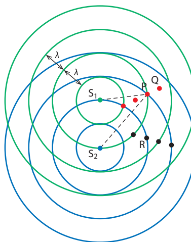
Figure 14.30: Wavefronts from two sources meet and interfere.
