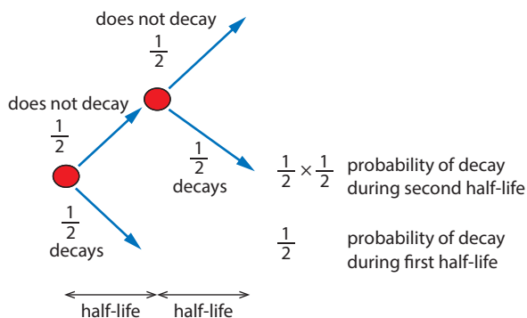
Figure 23.6: Tree diagram for nuclear decay.
