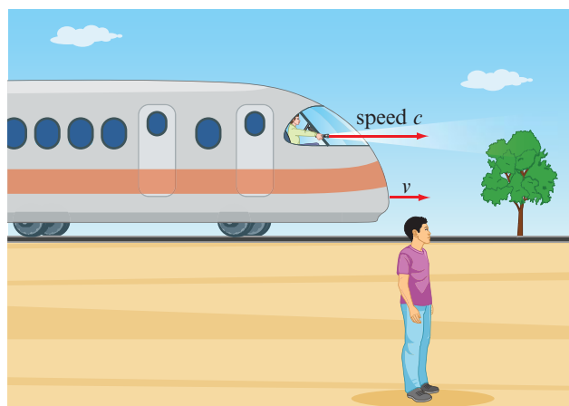
Figure 6.9: An observer in the train measures the speed of light to be c . An observer on the ground would then measure a higher speed, c + v .
