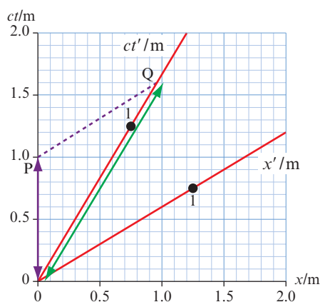
Figure 6.32: This clock shows ct = 1 at P .
