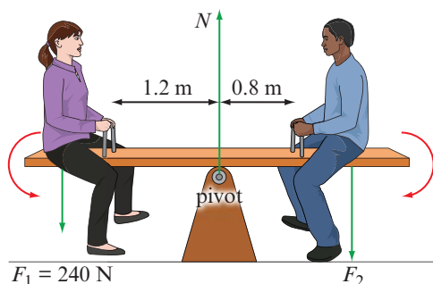
Figure 5.10: A see-saw in equilibrium.
