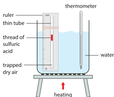
Figure 9.8: Apparatus for verifying the volume–temperature law.
