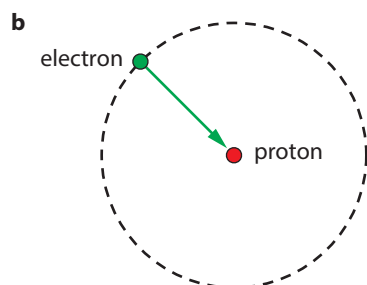
Figure 21.9: a Niels Bohr. b An electron orbiting a proton. The force on the electron is the electric force.
