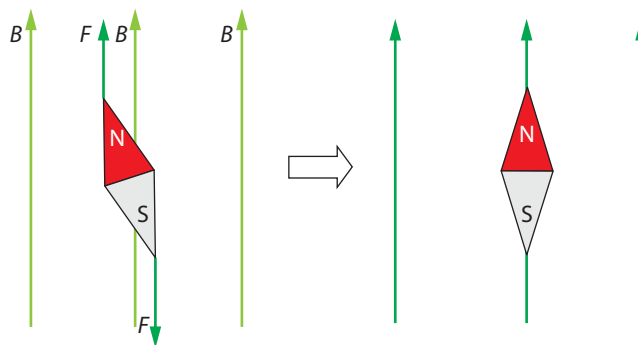
Figure 18.24: A magnetic needle in an external magnetic field experiences forces that will align it with the direction of the magnetic field. The direction of the needle (from its south to the north pole) gives the direction of the external magnetic field.
