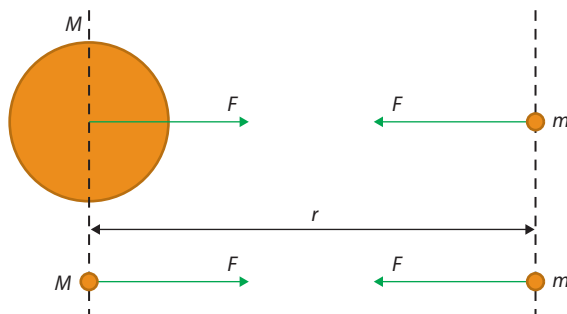
Figure 17.1: The mass of the spherical body to the left can be thought to be concentrated at its centre.
