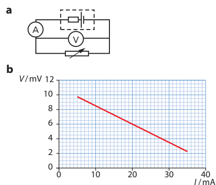
Figure 11.53: For worked example 11.19.
