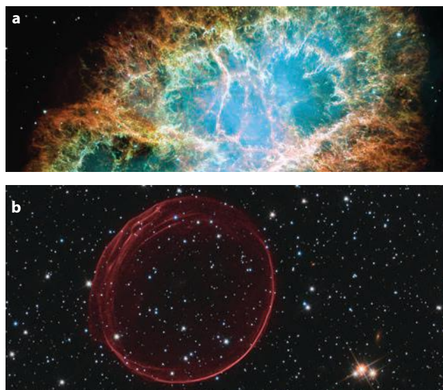
Figure 25.11: a The Crab nebula, the remnant of a supernova observed by the Chinese in 1054 and perhaps also by Native Americans. It was visible for weeks even during daytime. b This majestically serene bubble of gas is the remnant of a supernova that happened 400 years ago.
