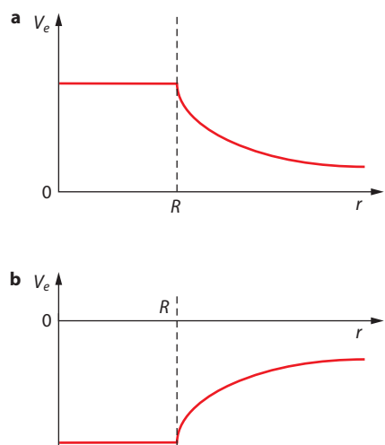
Figure 18.68: The electric potential is constant inside the sphere and falls off as \frac{1}{r} outside. Shown here are a a positively charged sphere and b a negatively charged sphere.
