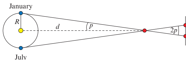
Figure 25.5: The earth (blue circles) in orbit around the sun. The star is observed from two positions six months apart.
