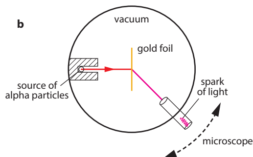
Figure 21.1: a The majority of alpha particles are slightly deflected by the gold foil. Very occasionally, large-angle scatterings take place. b The alpha particles are detected by the sparks of light they create when they hit a zinc sulfide screen in the microscope.
