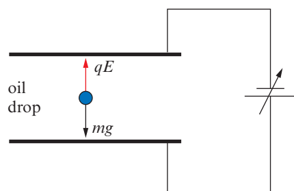
Figure 18.16: Schematic diagram of Millikan's apparatus.
