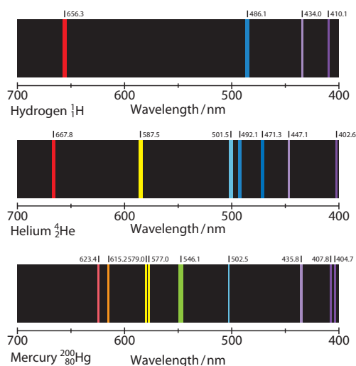
Figure 21.3: The emission spectra of hydrogen, helium and mercury vapour.
