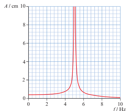
Figure 15.15: Graph showing the variation with driving frequency of the amplitude of driven SHM when the system is driven by an external periodic force and no damping. The natural frequency is 5 Hz here.
