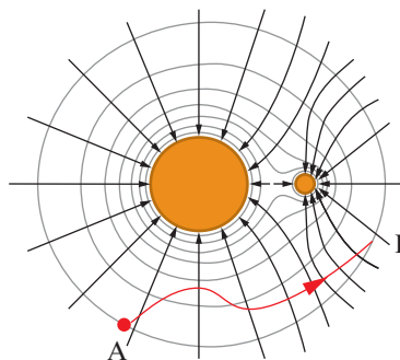
Figure 17.21: Zero work is done when moving a mass from one point to another on the same equipotential.
