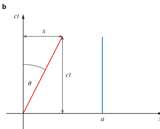
Figure 6.22: a The space and time co-ordinates of an event: x = 5.0 m and ct = 6.0 m. b The worldline of a particle at rest is the sequence of events showing the position of the particle at different times (blue line). A particle moving to the right has a worldline shown by the red line.
