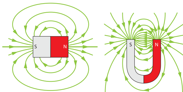
Figure 18.25: Magnetic field lines of a bar magnet and a horseshoe magnet. Notice that the arrows exit the north poles.
