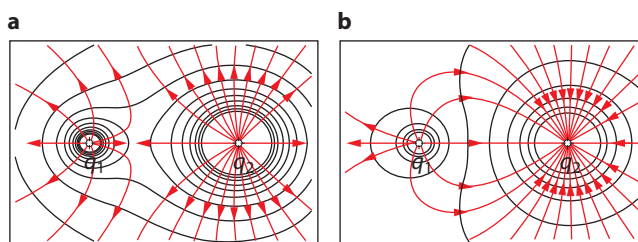
Figure 18.74: Field lines and equipotential surfaces for a two unequal charges of the same sign and b two unequal and opposite charges.
