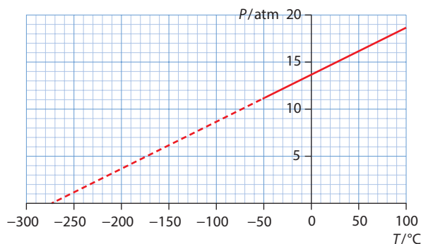
Figure 9.13: The graph of pressure against temperature is a straight line that, when extended backwards, again intersects the temperature axis at -273^\circ\text{C} .
