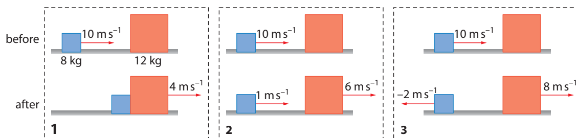
Figure 4.15: Momentum is conserved in these three collisions.
