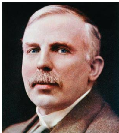
Figure 21.8: Ernest Rutherford.
