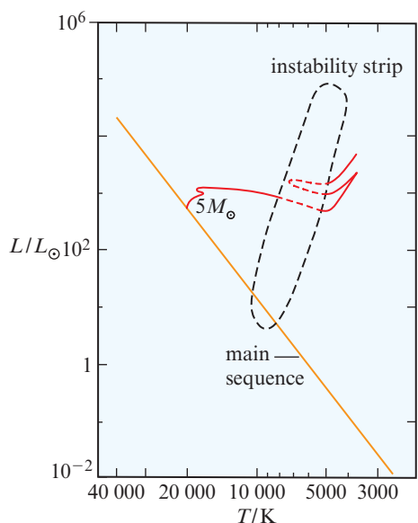
Figure 25.9: The instability region of the HR diagram.
