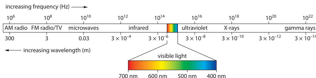
Figure 13.27: The electromagnetic spectrum.
