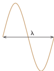
Figure 13.3: One full wave.
