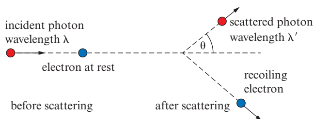
Figure 22.8: A photon incident on an electron scatters off the electron; the electron recoils.
