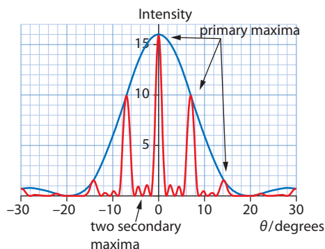
Figure 14.54: Intensity pattern for four slits.
