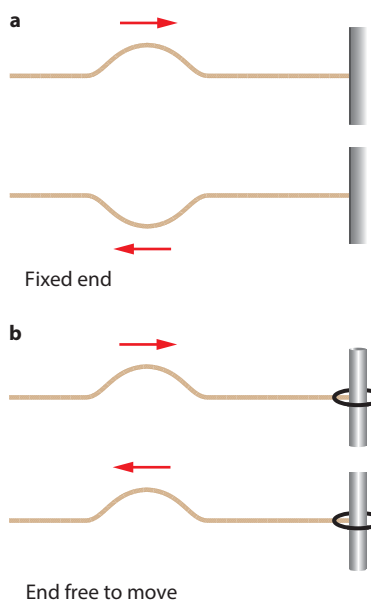
Figure 14.21: Reflection of a pulse from a a fixed end and b a free end. Notice the inversion in the case of the fixed end.
