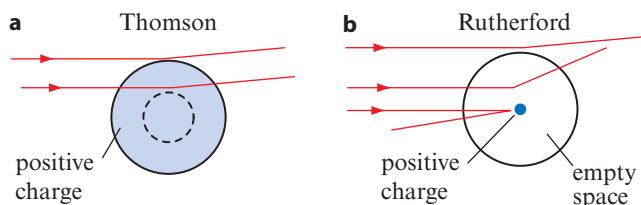
Figure 21.2: a We cannot get a large force out of the Thomson model, but b with a tiny nucleus we can.
