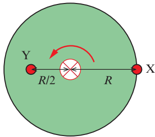
Figure 5.3: For worked example 5.3.
