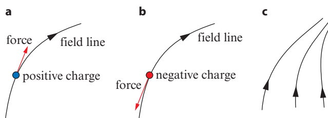
Figure 18.8: a The electric force on a positive charge is tangential to the field line in the direction of the arrow of the field line. b The force on a negative charge is tangential to the field line in a direction opposite to the arrow. c The density of field lines increases as we move towards the top of the page and so the electric field strength increases.
