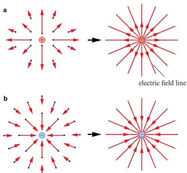
Figure 18.6: The electric force experienced by a a positive test charge at various positions near a positive and b a negative point charge. The diagrams on the right show the electric field lines.
