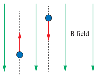
Figure 19.14: When the velocity is parallel or anti-parallel to the magnetic field the force is zero.
