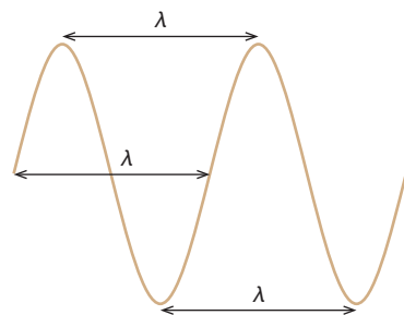
Figure 13.4: Three distances that all give the wavelength.
