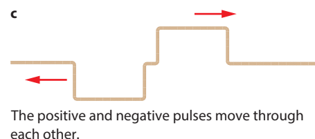
Figure 14.19: The superposition of a positive and a negative pulse.
