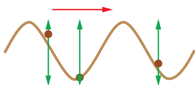
Figure 13.6: Particles in the medium move strictly at right angles to the direction of energy transfer.
