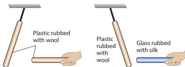
Figure 18.1: Two simple experiments to investigate properties of electric charge.
