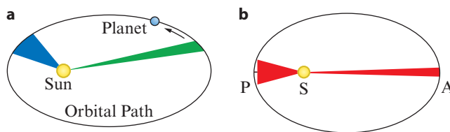
Figure 17.8: a In equal times, the line joining the planet to the sun sweeps out equal areas. b The special case when the planet is at perihelion (P) and aphelion (A).
