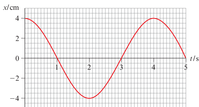
Figure 12.33: Displacement versus time graph.
