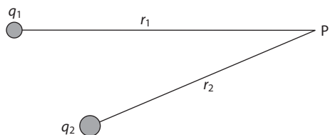
Figure 18.67: The potential at P is found by finding the potential there from the first charge, then finding the potential from the second charge, and finally adding the two.
