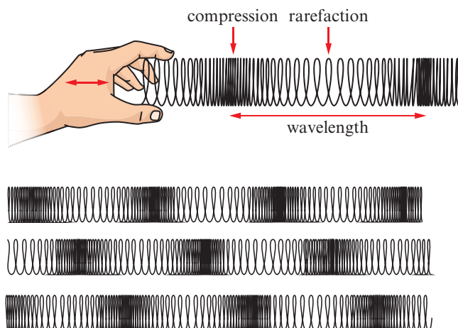
Figure 13.12: A longitudinal wave in which the medium moves parallel to the direction of energy transfer.
