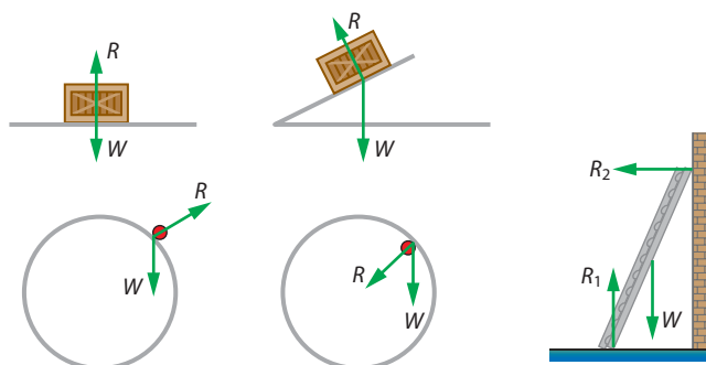
Figure 2.6: Examples of normal forces, R .
