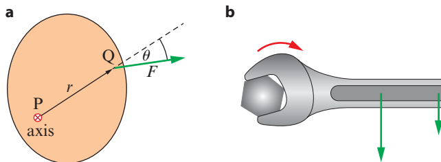
Figure 5.6: a The force tends to rotate the body about the axis in the clockwise direction. This is because the force has a torque about that axis. b A wrench turning a screw is a real-life application of torque. A smaller force further from the axis has the same turning effect as a larger force closer to the axis.
