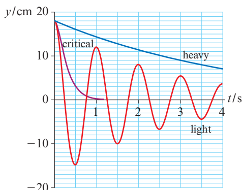
Figure 15.17: Light, critical and heavy damping.
