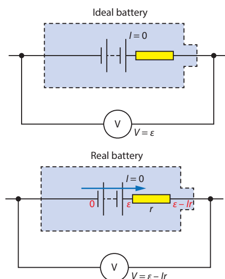
Figure 11.52: The potential difference across the terminals of a battery is equal to the emf when there is no current in the circuit. It is less than the emf when there is current.
