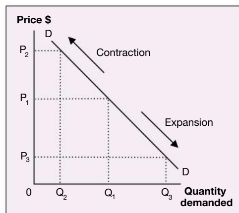
Figure 6.3 – Expansions and contractions in demand
