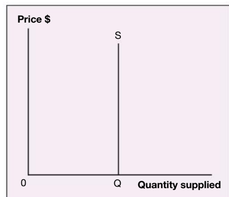
Figure 7.7 – Perfectly inelastic supply
