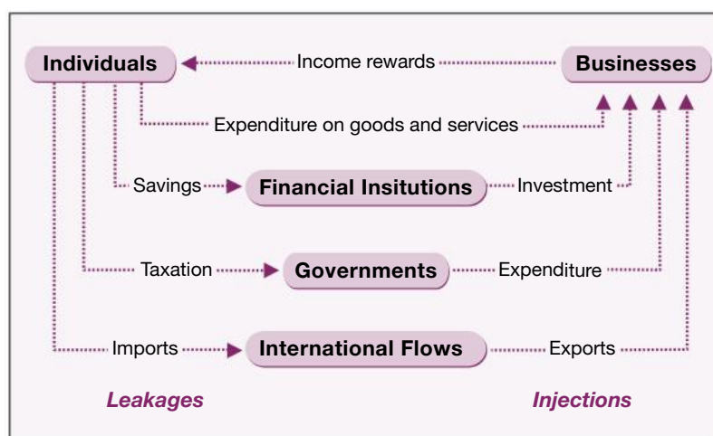
Figure A.3 – Equilibrium and the circular flow model
