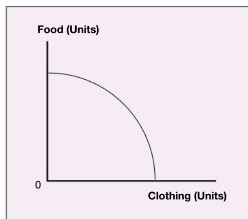
Figure A.2 – Production possibility frontier
