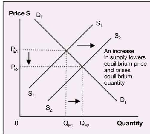
Figure 8.6 – An increase in supply
