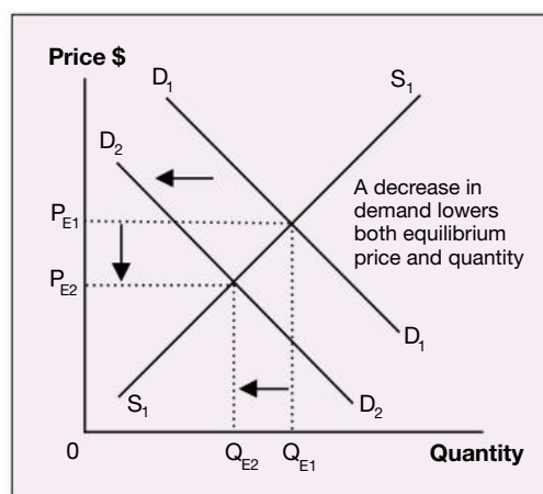
Figure 8.5 – A decrease in demand
