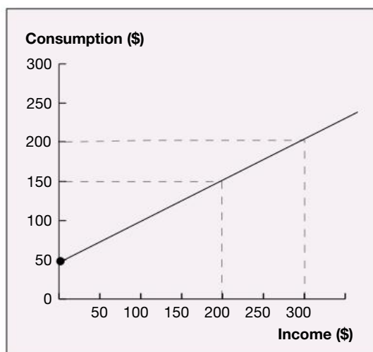
Figure 4.2 – The consumption function
