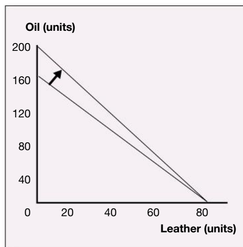
Figure 1.3 – An improvement in the technology of oil production
