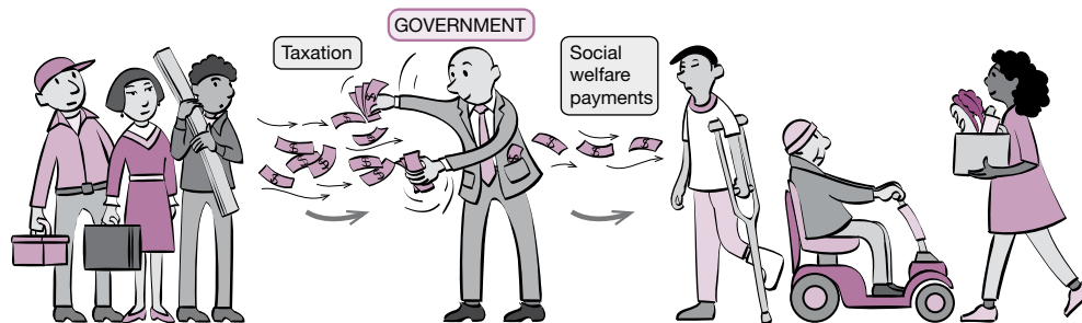
Figure 15.5 – The redistribution of income
