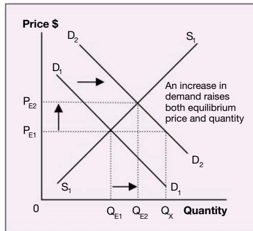
Figure 8.4 – An increase in demand
