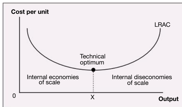
Figure 5.3 – The long-run average cost curve
