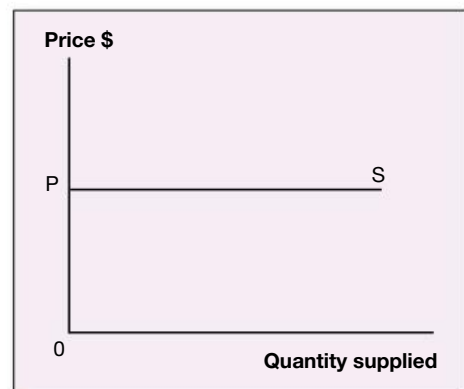
Figure 7.6 – Perfectly elastic supply
