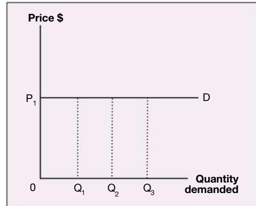
Figure 6.8 – Perfectly elastic demand
