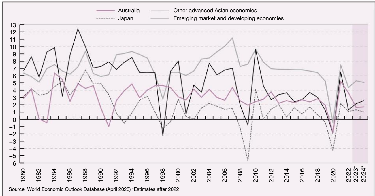
Figure 3.2 – GDP growth, selected economies
