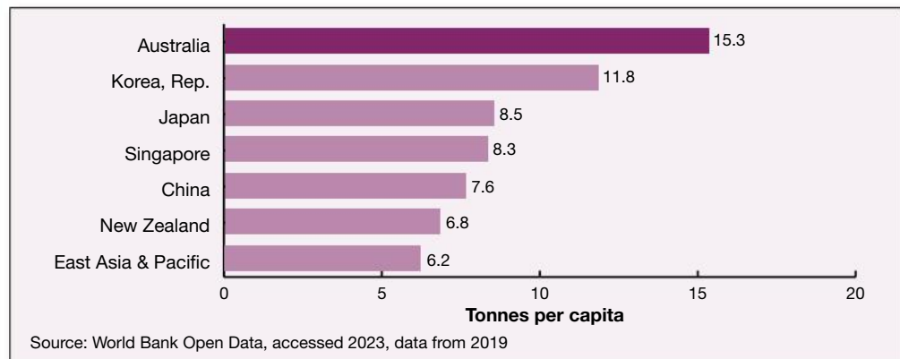
Figure 3.6 – Carbon dioxide emissions, selected economies
