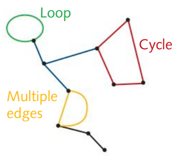
Graph 3: not a tree
