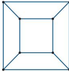
Graph 2 Cube
