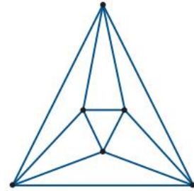
Graph 3 Octahedron
