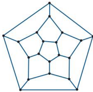
Graph 4 Dodecahedron
