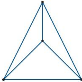
Graph 1 Tetrahedron
