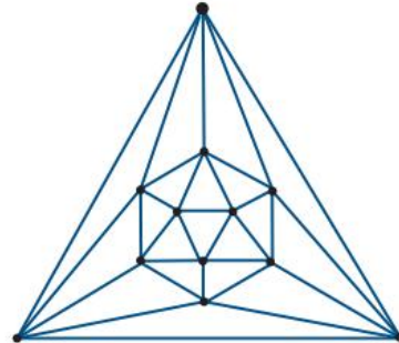
Graph 5 Icosahedron
