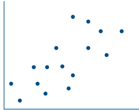
Moderate positive association
