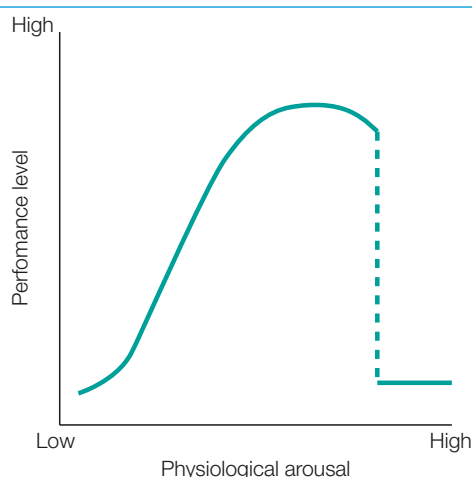
Figure 3.6.19: Catastrophe theory.
