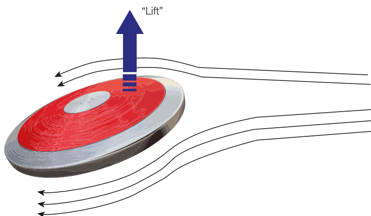
Figure 1.3.40: The discus 'lifts' as it moves from an area of high to low pressure.
