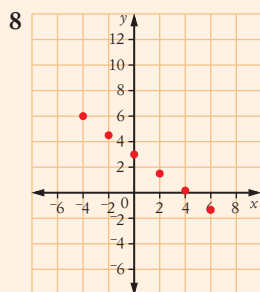
Decreasing linear function
