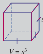
Cube
