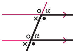
corresponding angles
