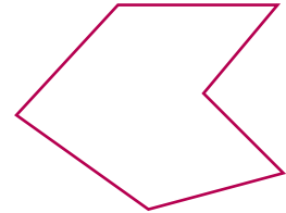
Non-convex polygon
