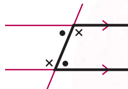
co-interior angles
