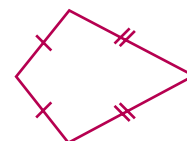
Kite
