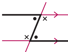
alternate angles
