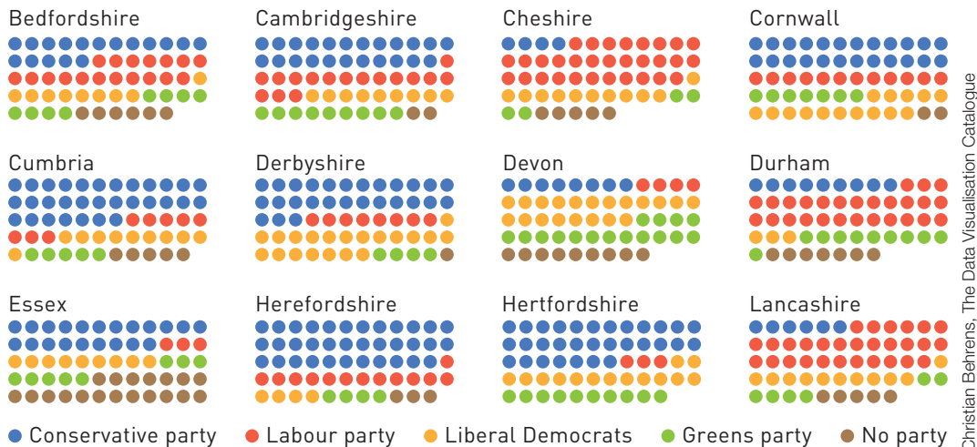
FIGURE 7.16 Matrix visualisation
