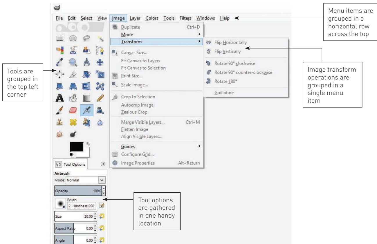
FIGURE 6.18 GIMP interface
