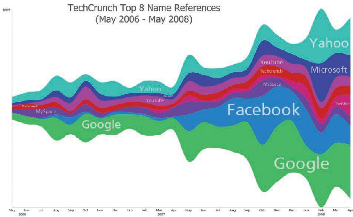
FIGURE 7.13 Time visualisation
