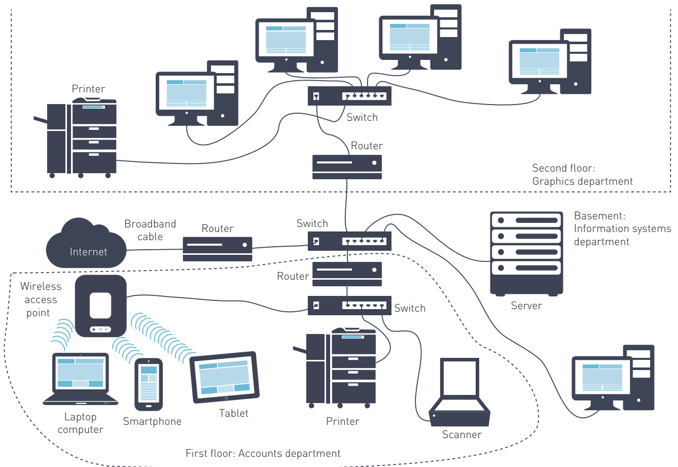
FIGURE 3.9 How a router can connect two LANs and provide internet access to both networks.
