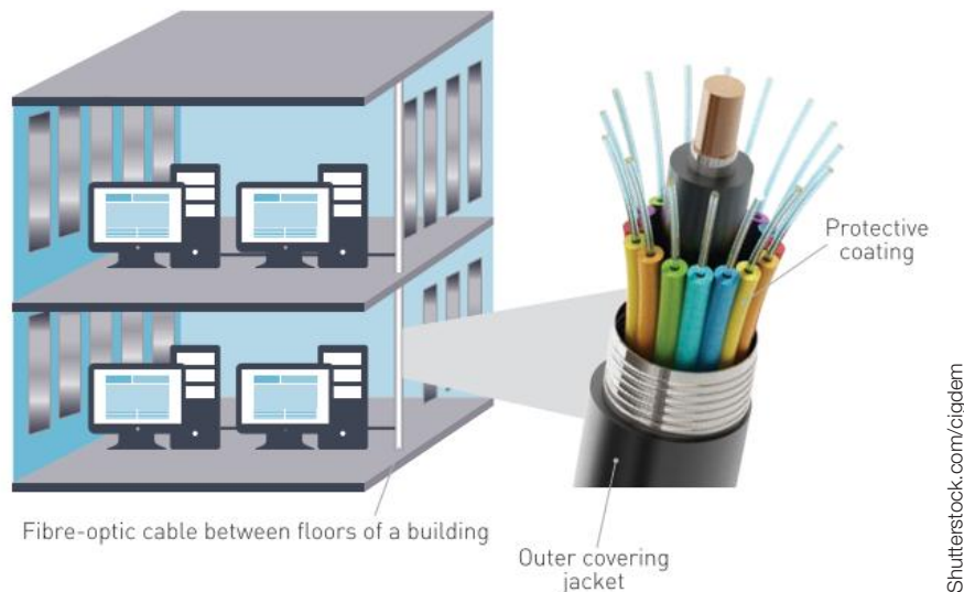
FIGURE 3.31 A fibre-optic cable consists of hair-thin strands of glass or plastic that carry data as pulses of light.
